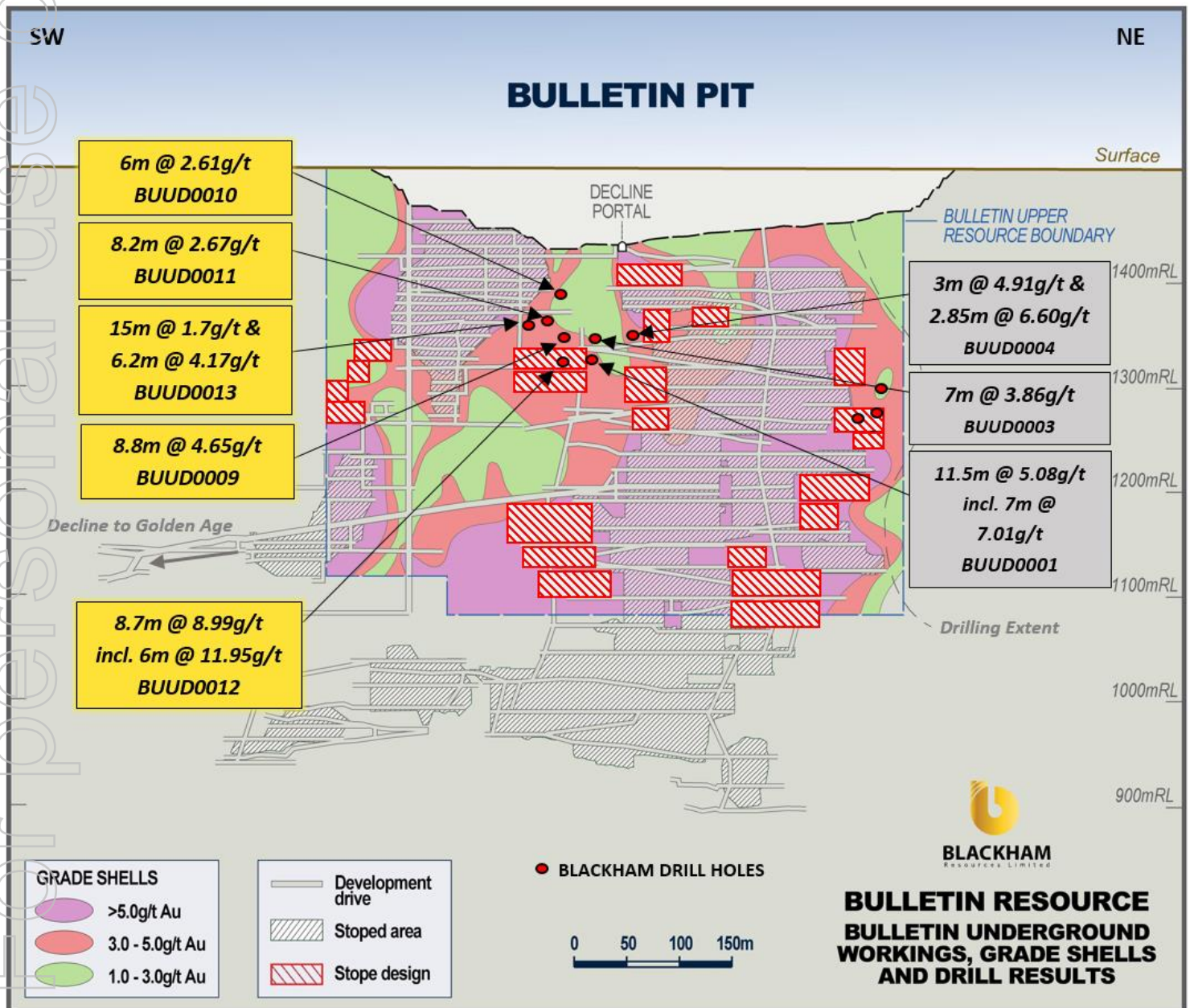
Fig 1. Long-section looking North West of Bulletin underground workings, grade shells, designed stopes, and recent drill intercepts.
