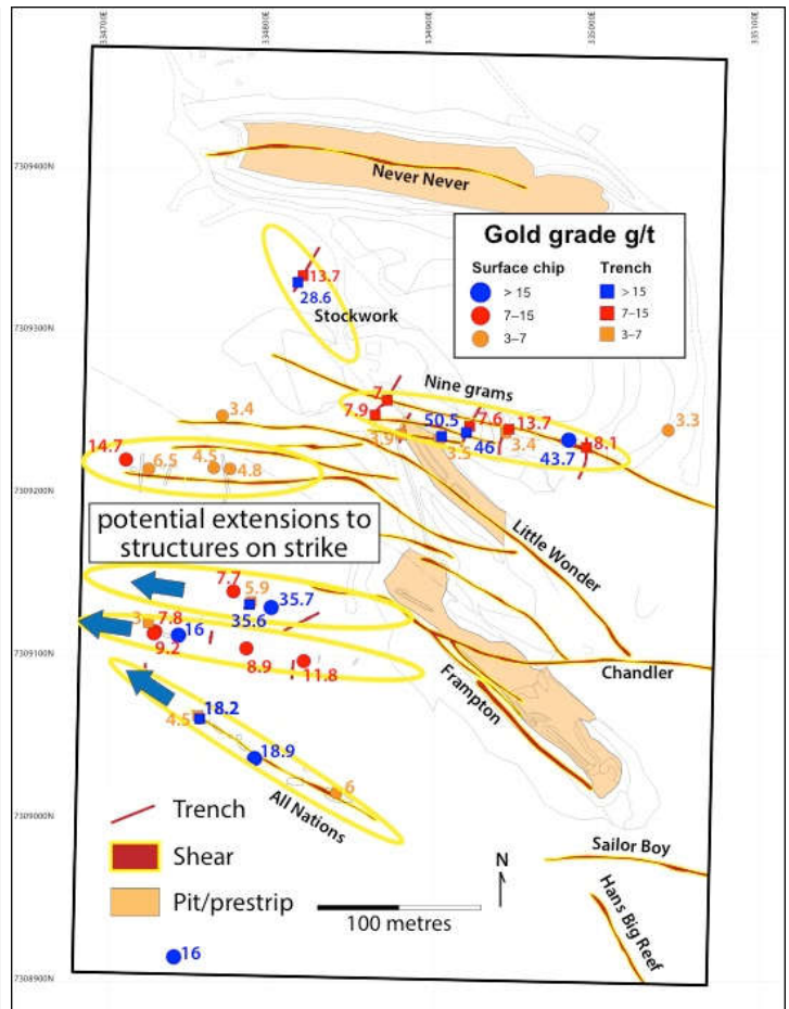
Figure 5: Trench and rock chip locations.
