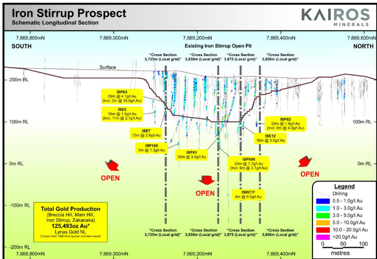
Figure 3 – Schematic Long Section of the Iron Stirrup Deposit
