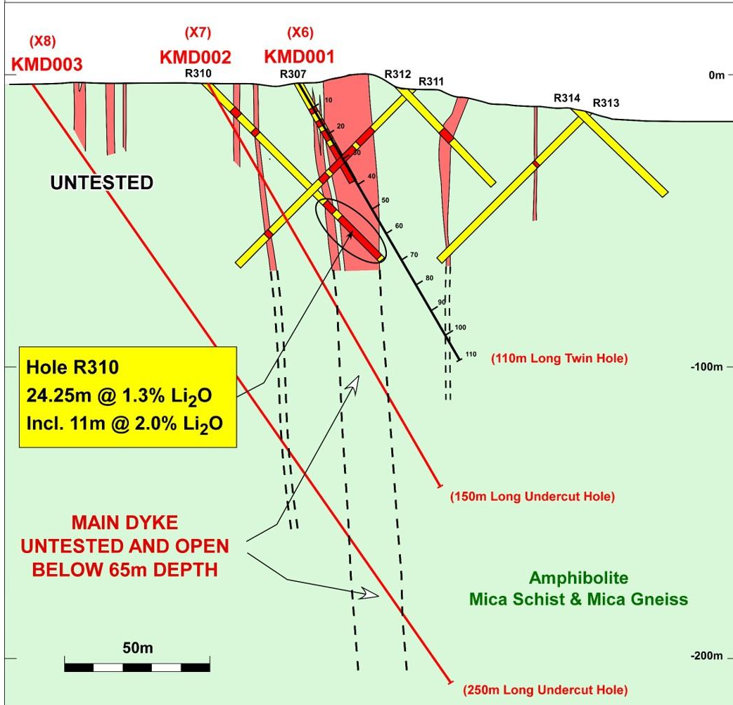
Diagram showing a section through the Kietyönmäki deposit on the traverse of KMD001.
