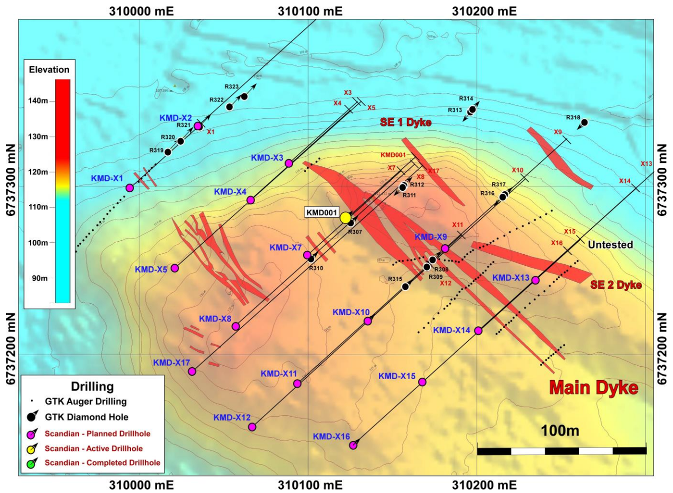
Diagram showing a plan of the Kietyönmäki deposit area and the location of historical and proposed drill holes. KMD001 is shown in yellow.
