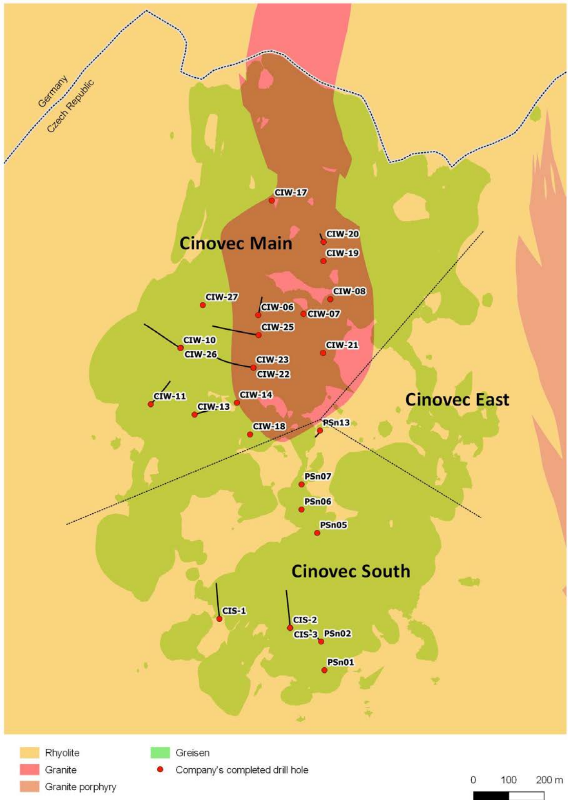
Figure 1 - A geological map showing the Company's drill holes (with angled holes traces projected to surface) against surface geology and subsurface greisen bodies projected to surface (in green). Historic UG workings and drill holes not shown.
