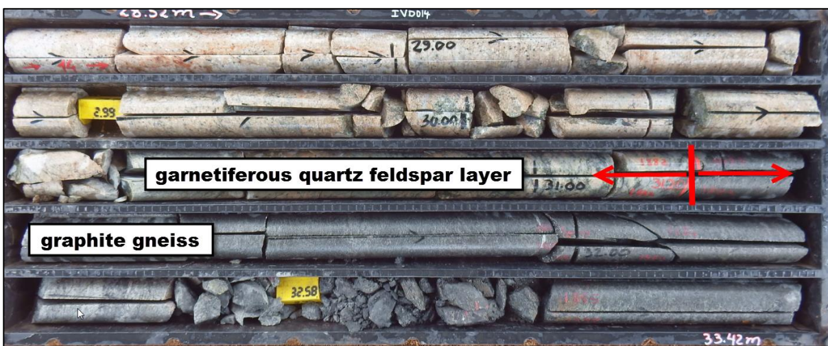
Figure 6: Garnetiferous quartzo-feldspathic marker layer and graphitic gneiss in IVD014 Mineralisation zone 2
