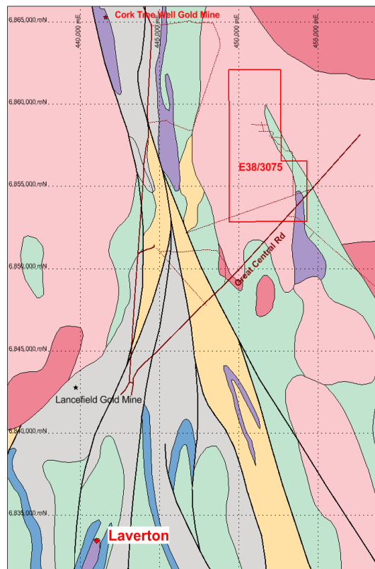
Figure 2 – Tenement Location with Underlying Geology
