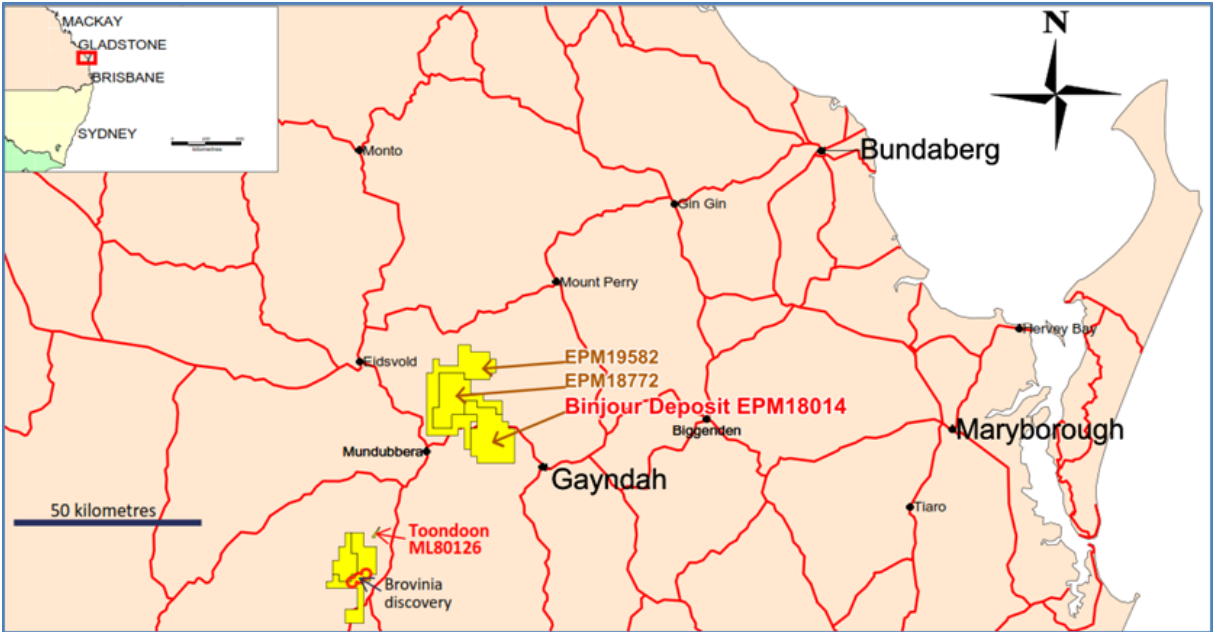
Figure 1: Locations of ABx’s Binjour Project and roads infrastructure. Map shows Binjour deposit, granted ML 80126 at Toondoon and the bauxite discovery at Brovinia. The distance from Binjour to Bundaberg Port is 115kms.
