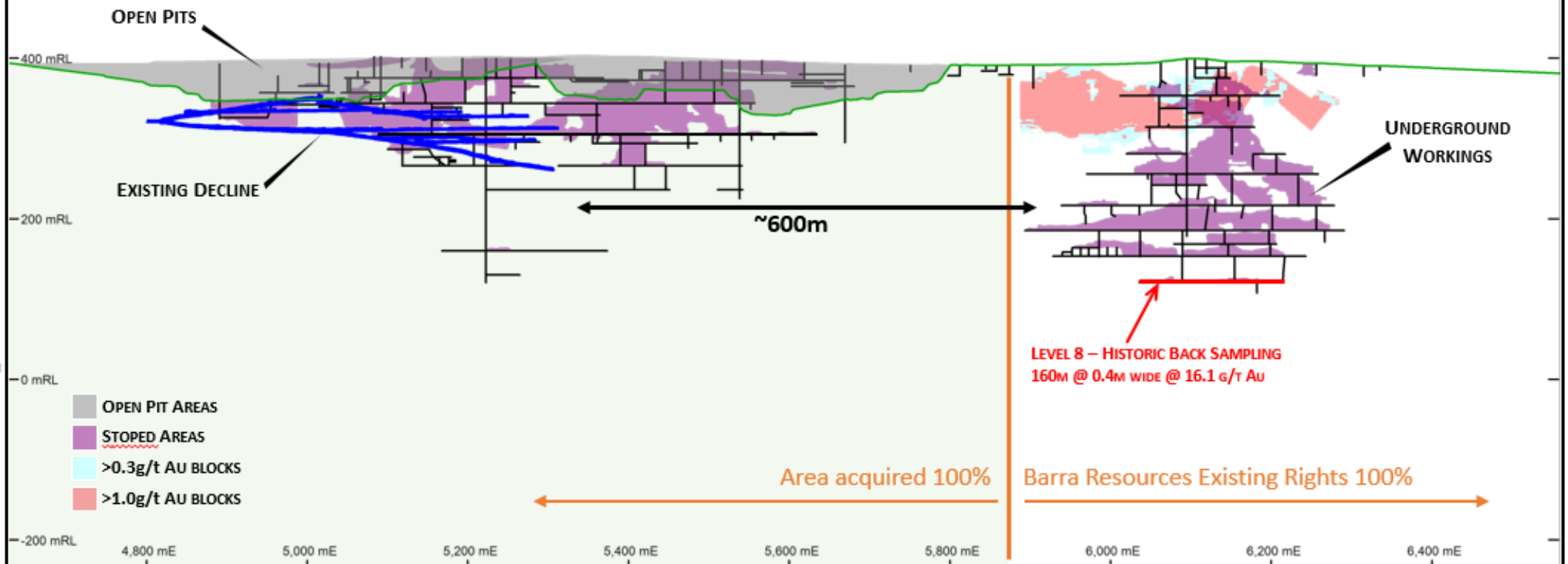
Figure 2: Burbanks Mining Centre Schematic Long Section
