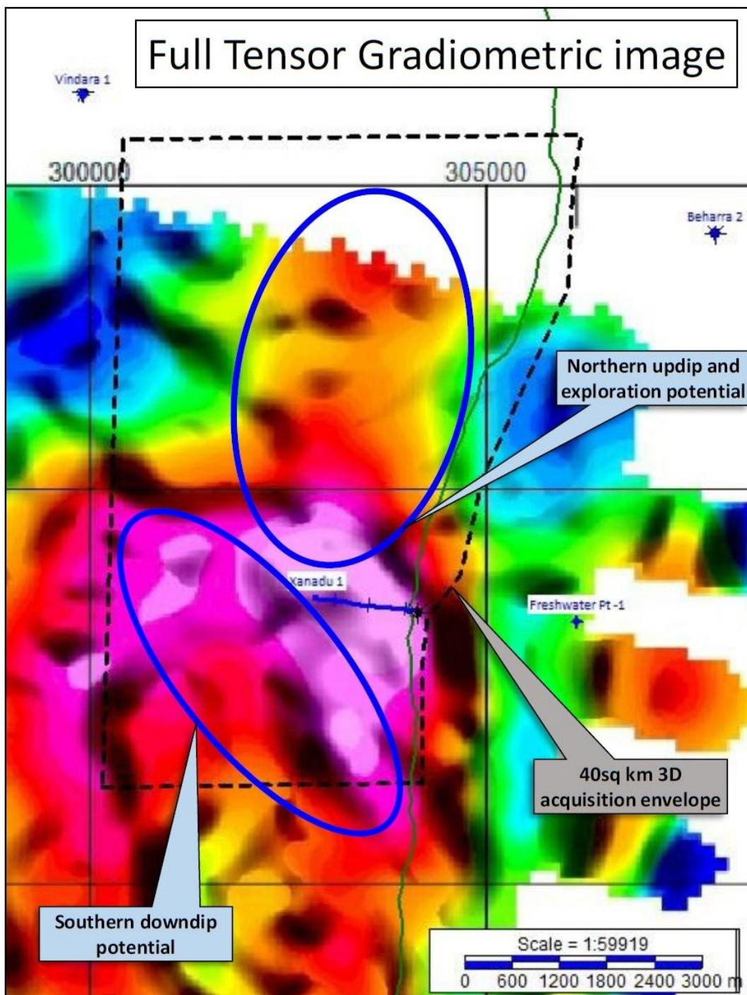
Figure 1. Xanadu 40 KM 2 3D Seismic Survey Acquisition area overlying a full tensor gradiometric image, highlighting up-dip and down-dip potential at Xanadu.
