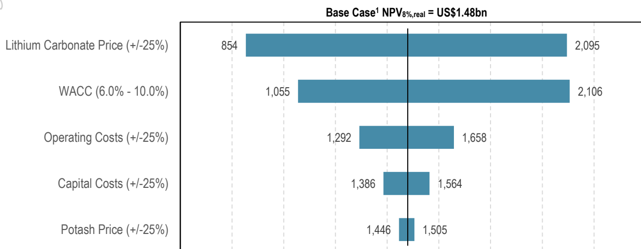
Figure 2: Financial Sensitivity
