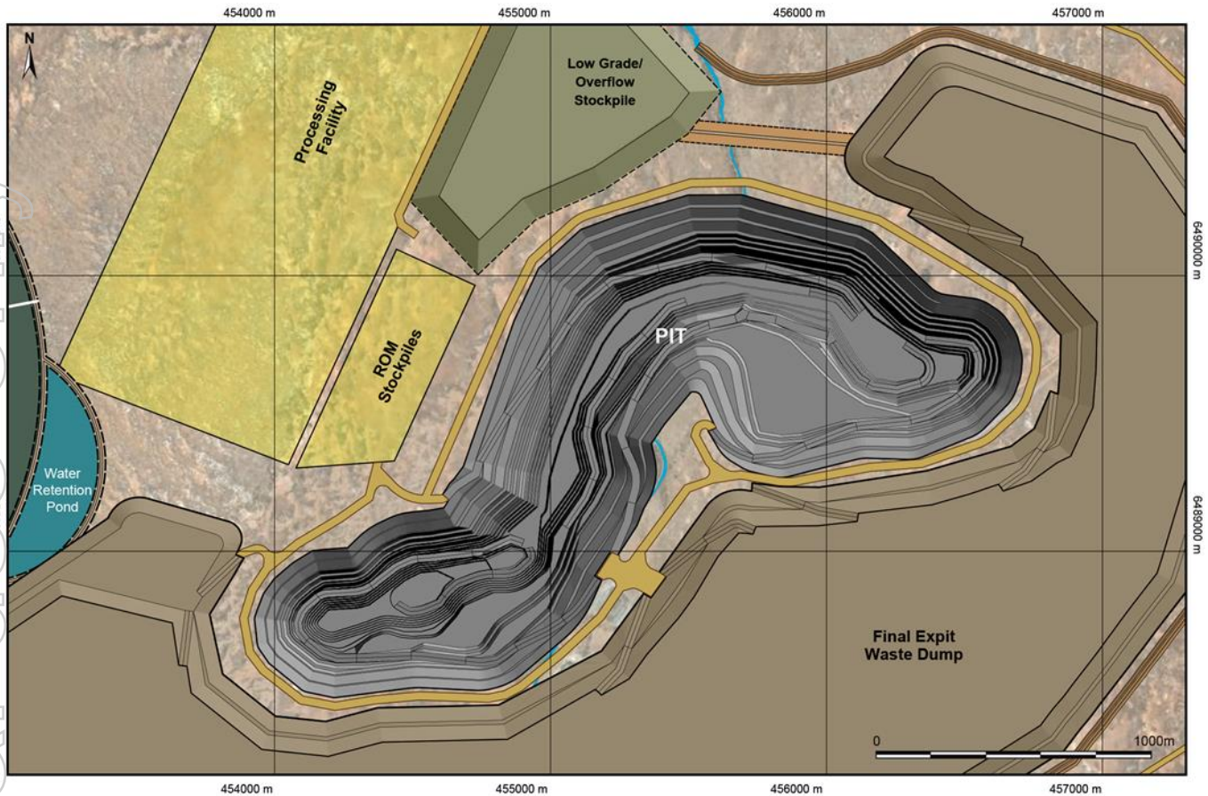
Figure 2 Kalkaroo ultimate open pit design.
