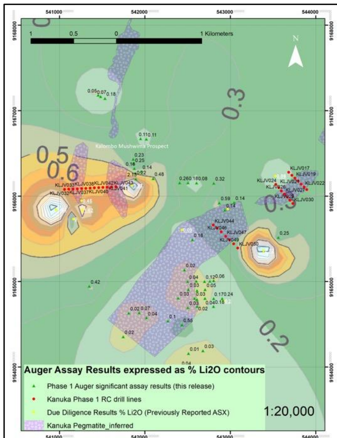
Figure 7: Highlighting gridded assay results (Inverse distance to a power) of the new Auger bedrock geology results, combined with previous ASX Due Diligence results (2017) and inferred pegmatites Phase 1 RC Drilling. Contouring was conducted using 74 sample points.
