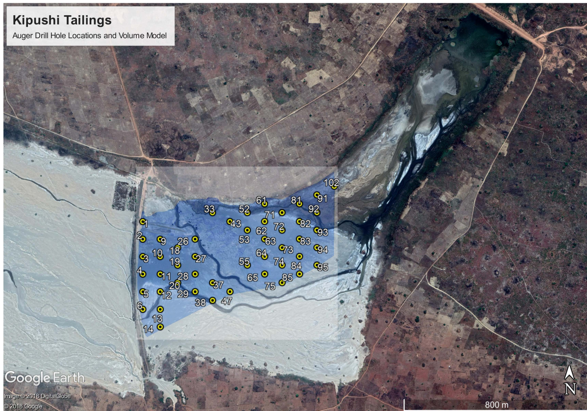
Figure 2: Drill Hole Locations overlain with volume model in blue.
