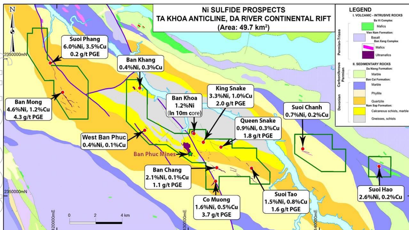
Figure 9: Ta Khoa dome geology prospective for multiple magmatic nickel sulfide deposits (refer to Table two for trenching results)
