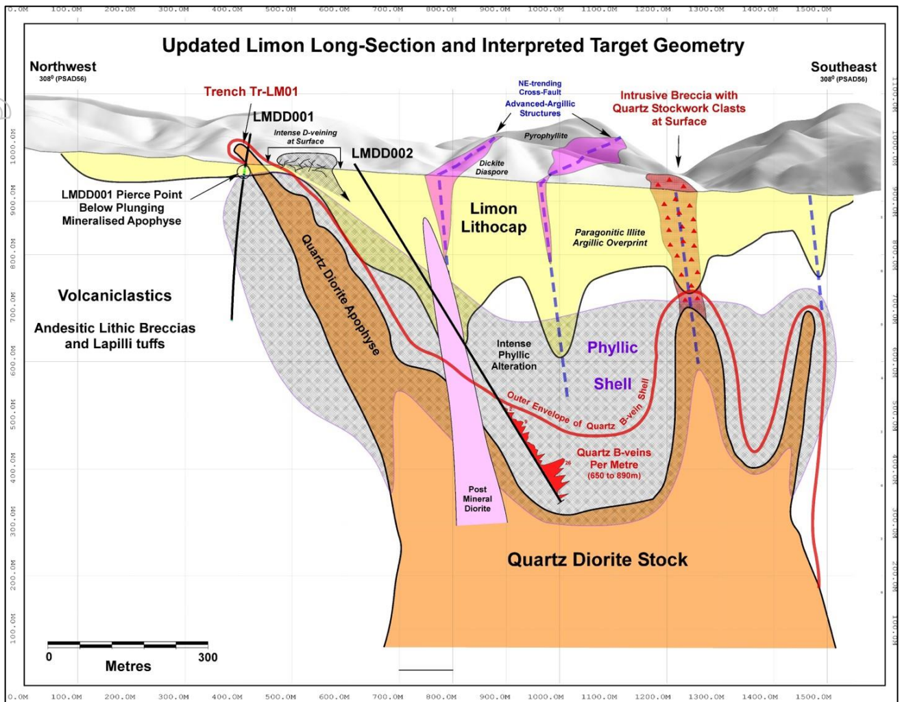
Figure 2: Schematic long-section showing the location of holes LMDD001 and 002. The upper parts of the target zone are within and surrounding the Quartz Diorite stock (within the red line outline) and will vary in depth in 3-D. Follow-up drilling will determine its geometry.
