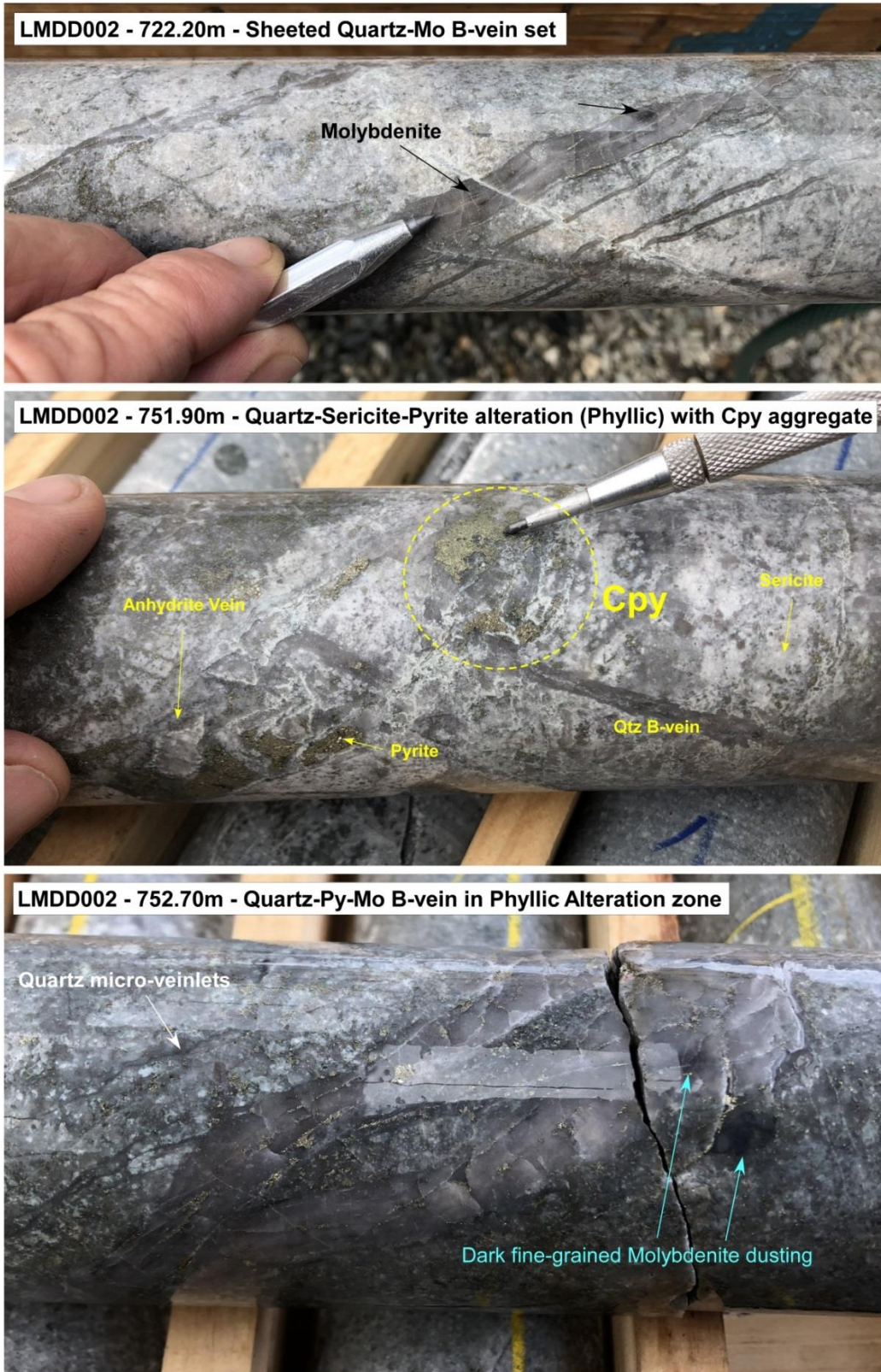
Plates 2-4 – Variety of porphyry B-vein textures seen in LMDD002 (Cpy = chalcopyrite).
