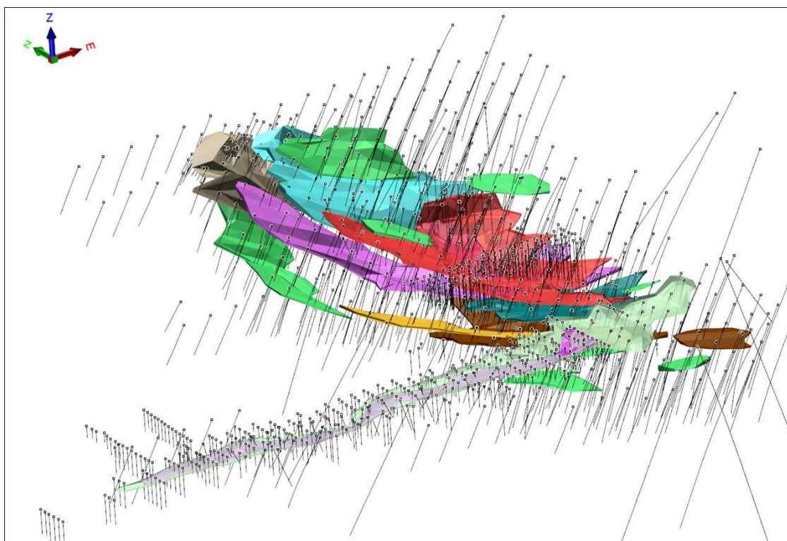
Figure 9 – Tampia drilling and lode domains
