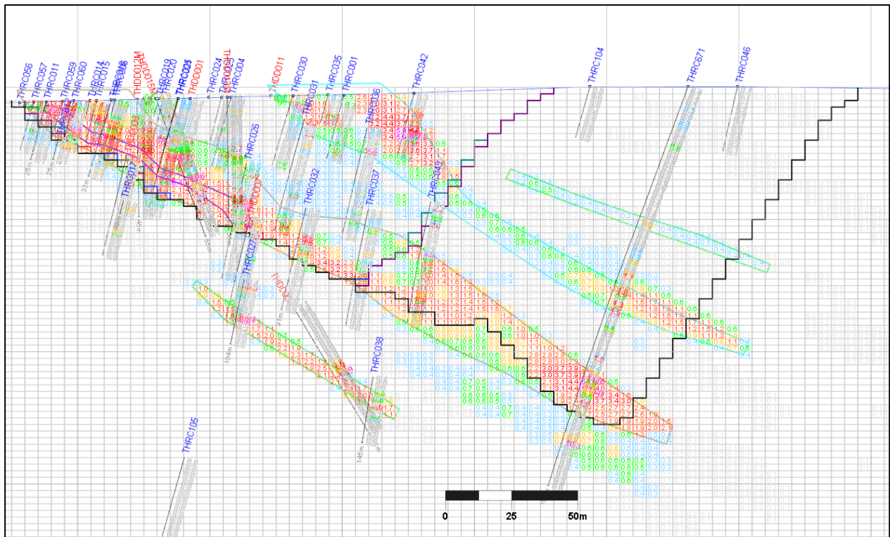
Figure 7 - Pit Optimisation results showing the difference between an A$1,800/oz and 10% improvement in bottom-line metric optimisation, in the northern part of the open pit where the impact is greatest
