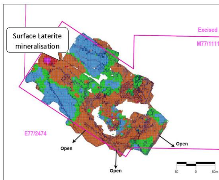
Figure 19 - Plan view - Symes Find Resource model
