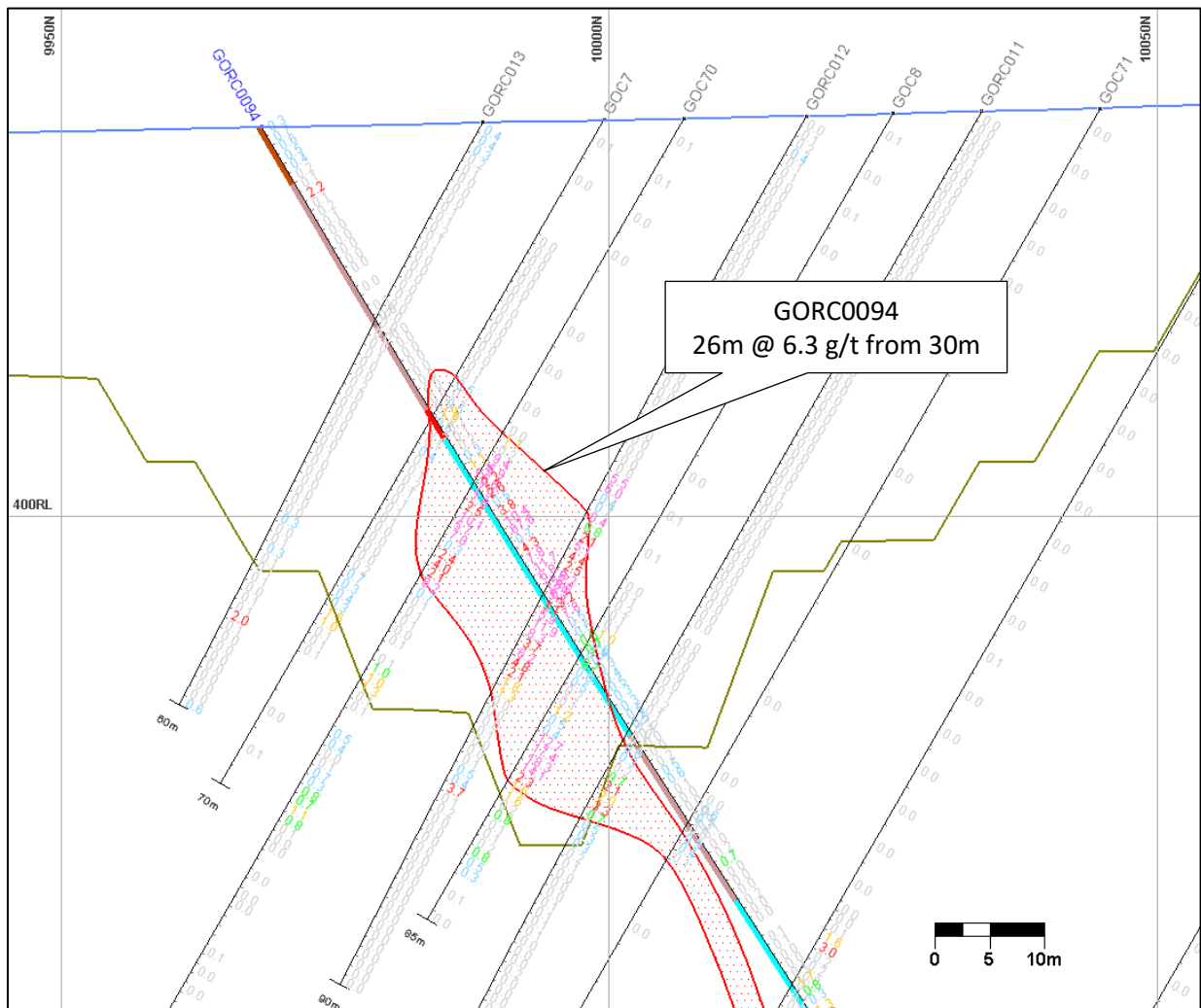
Figure 17 - Golden Orb local cross-section looking East
