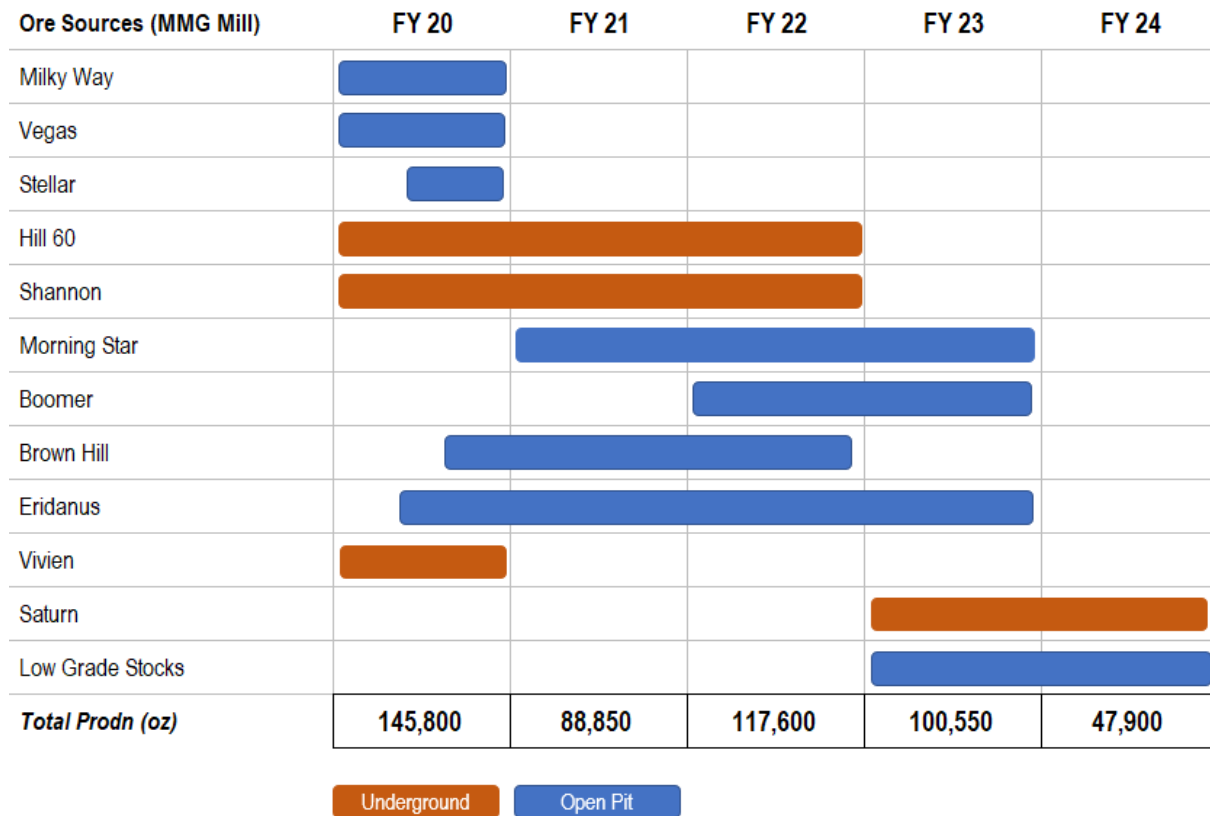
Figure 2 – Milling schedule by source at Mt Magnet
