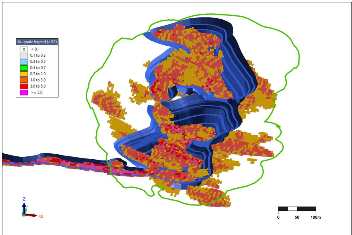
Figure 10 – Regularised block model (>0.7g/t) and initial open pit design with EXU pit outline in green
