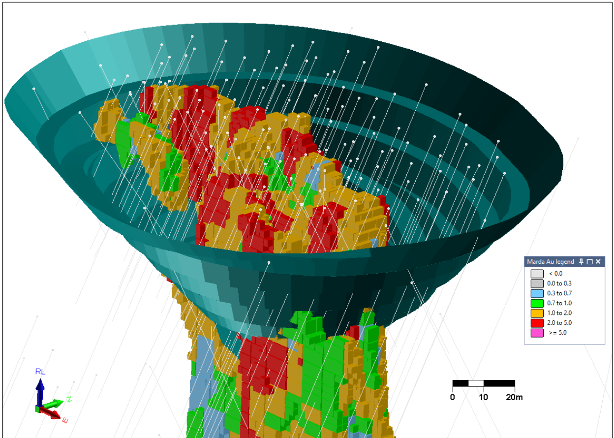
Figure 18 - Dolly Pot Drilling, Resource Model and Pit Design
