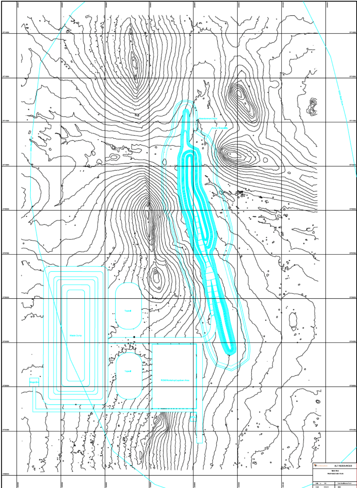
Figure 1: Tim's Find pit shell and site plan over the Digital Terrain Model
