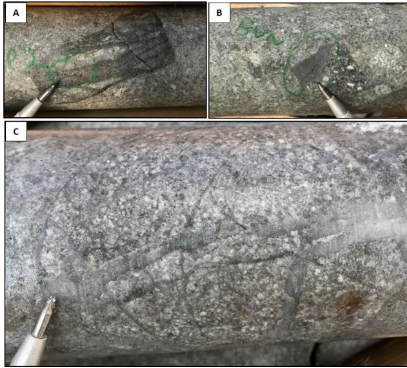
LMDD004 125-135m: Examples of porphyry clasts containing B, A and M type porphyry stockwork veining hosted in breccia pipes that have been ripped up from underlying diorite porphyry. A) Dense quartz B-veins in altered quartz diorite porphyry B) Fragment of a porphyry-related B-vein in a clast within a breccia pipe. C) Large 15cm clast of quartz B-vein stockwork (porphyry-related) in a breccia pipe.
