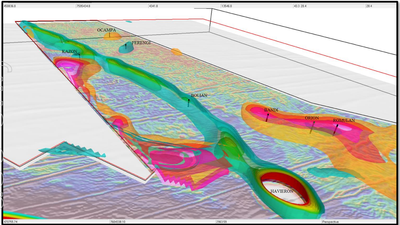
Figure 3: Armada Project, Paterson Ranges - 3D Inversion Results for Aeromagnetic/Gravity - Primary Target/Potential Deep Drill Holes Highlighted. Warm colours gravity inversion shells and green/cooler colours magnetic inversion shells (with exception of Havieron which is an intense magnetic high). This shows the top seven targets.
