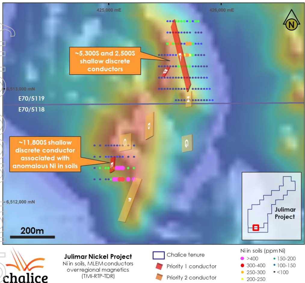
Figure 13. Julimar Nickel Project EM targets and soil geochemistry over regional magnetics.
