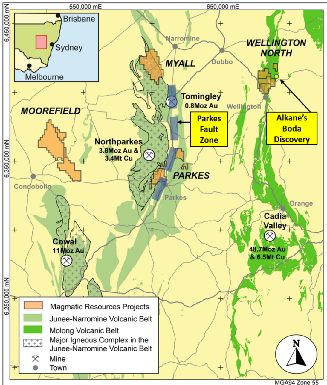
Figure 2: Location of Magmatic's projects in the East Lachlan, NSW showing mines and metal endowment 1
