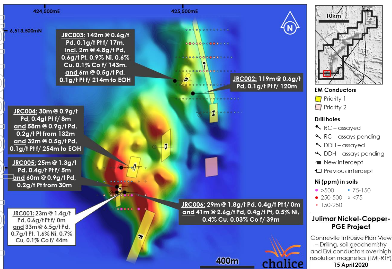
Figure 1. Gonneville Intrusive Plan View – Drilling and EM conductors over high-resolution magnetics.
