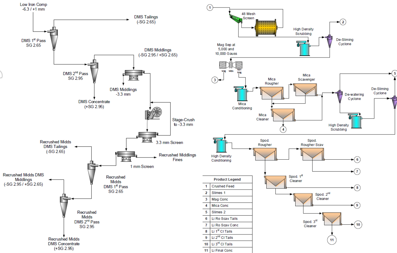
Figure 1 – DMS and Locked-Cycle Spodumene Flotation Testwork Flowsheets
