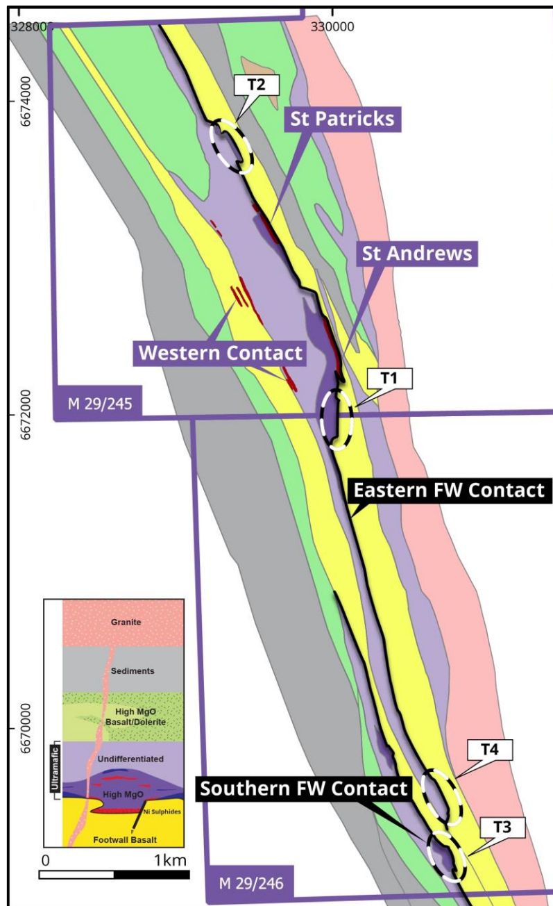
Figure 1 – Geological interpretation of the Saints Nickel Project showing the location of T2 and the other channel target areas (T1, T3 & T4)
