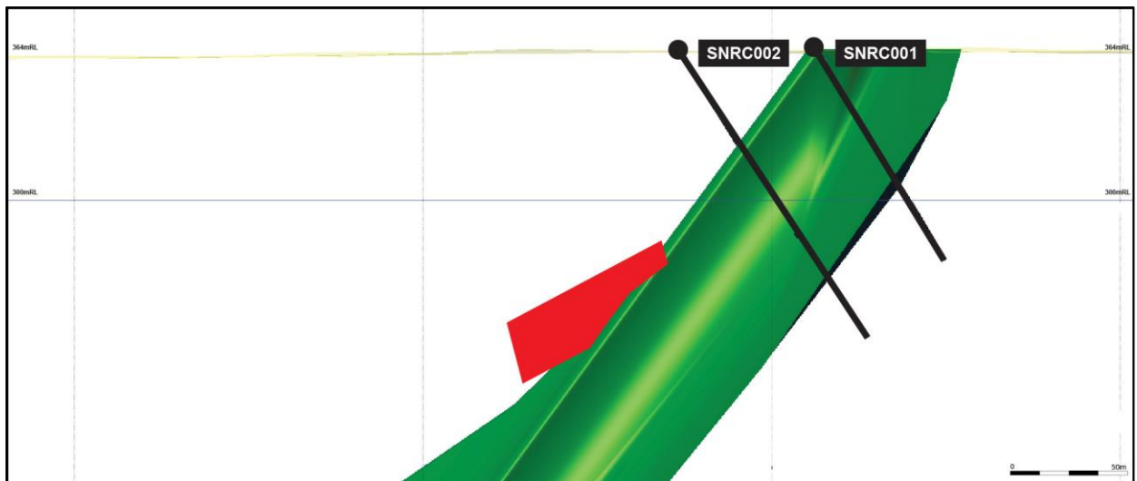
Figure 3 – 3D Cross-section at 6673720mN ± 60m through the T2 channel target area showing the location of the strong DHEM conductor (red plate) and completed RC drill-holes in relation to the modelled basal Eastern Footwall Contact (green). View is looking to the north
