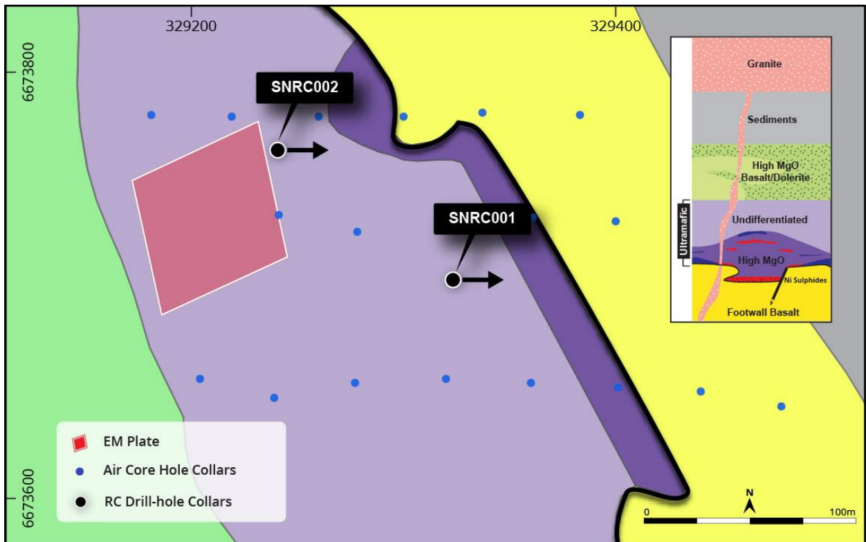
Figure 2 – Zoom of the T2 channel target area showing the location of the completed RC drill-hole collars and projection of the modelled DHEM conductor (plate) in relation to the interpreted geology
