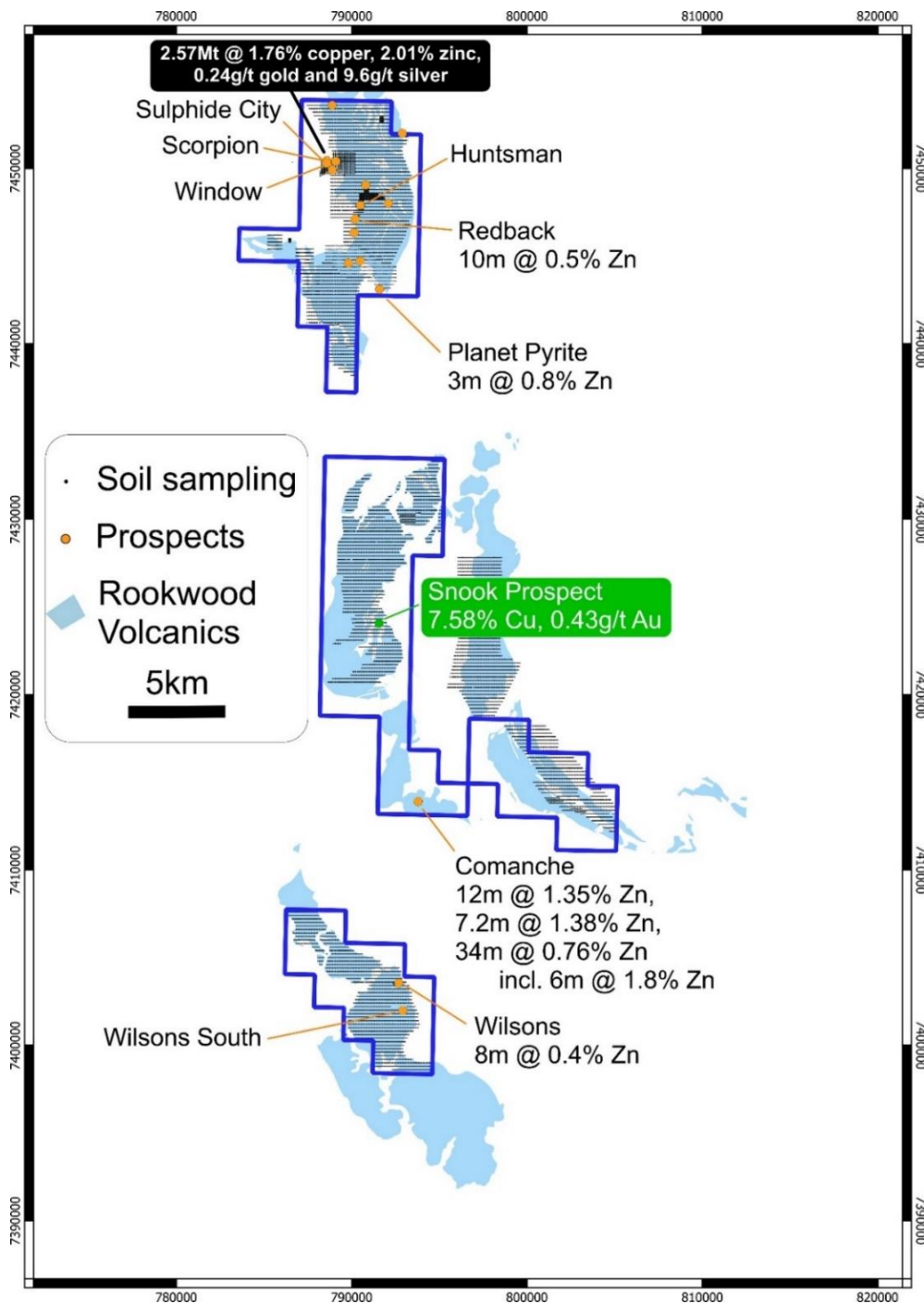
Figure 8: Develin Creek Prospects and Geochemical Anomalies
