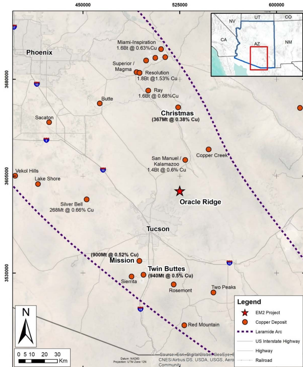
Figure 1 Location of Oracle Ridge Copper Project and other major copper mines/deposits in southern Arizona with Copper endowments. Mines with significant skarn-hosted mineralisation highlighted.
