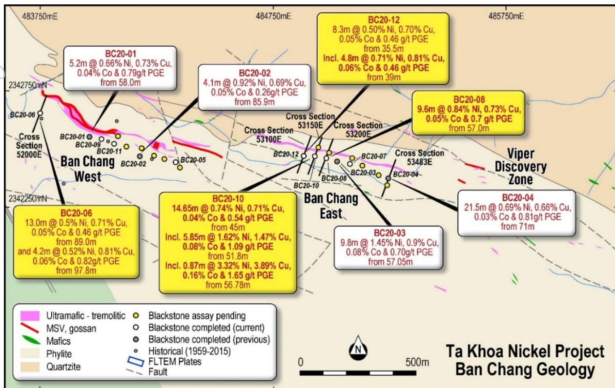
Figure 1: Ban Chang Geology
