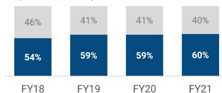
Automotive Sales Split: ICE vs Non-ICE (Revenue %, FY18-21)
