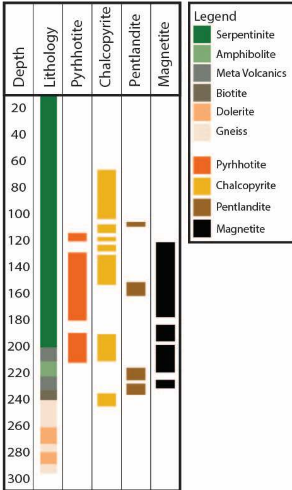
Figure 7 Mineralogical log for Sortekap drill-hole SODD001.
