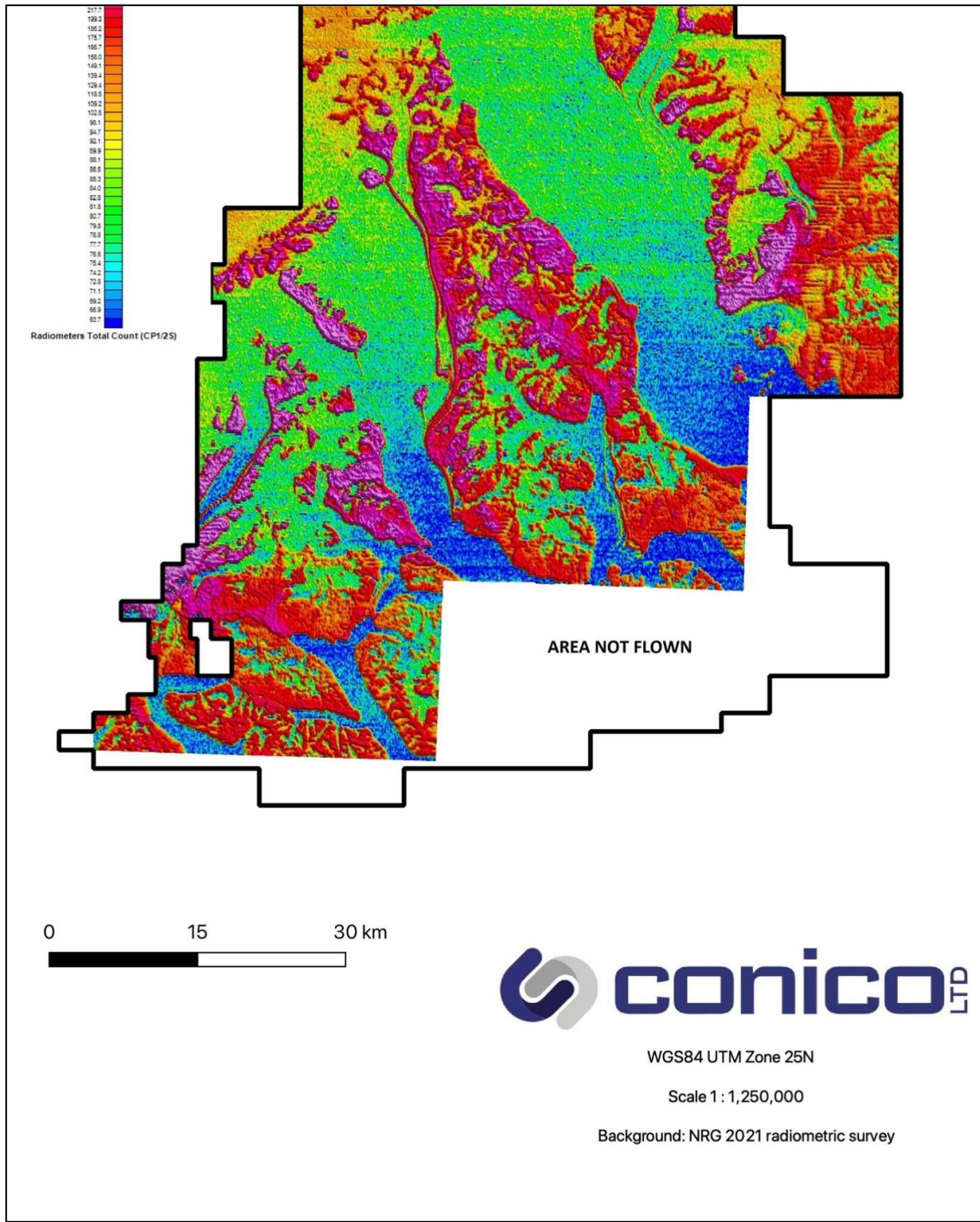
Figure 9 The newly completed NRG heli-borne radiometric survey.
