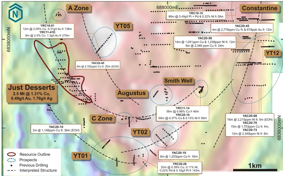
Figure 2 – Yuinmery Base Metal Deposits, Prospects and Drill Collar Locations Base Image 2009 VTEM ch25_1641us_NEshade Geophysics
