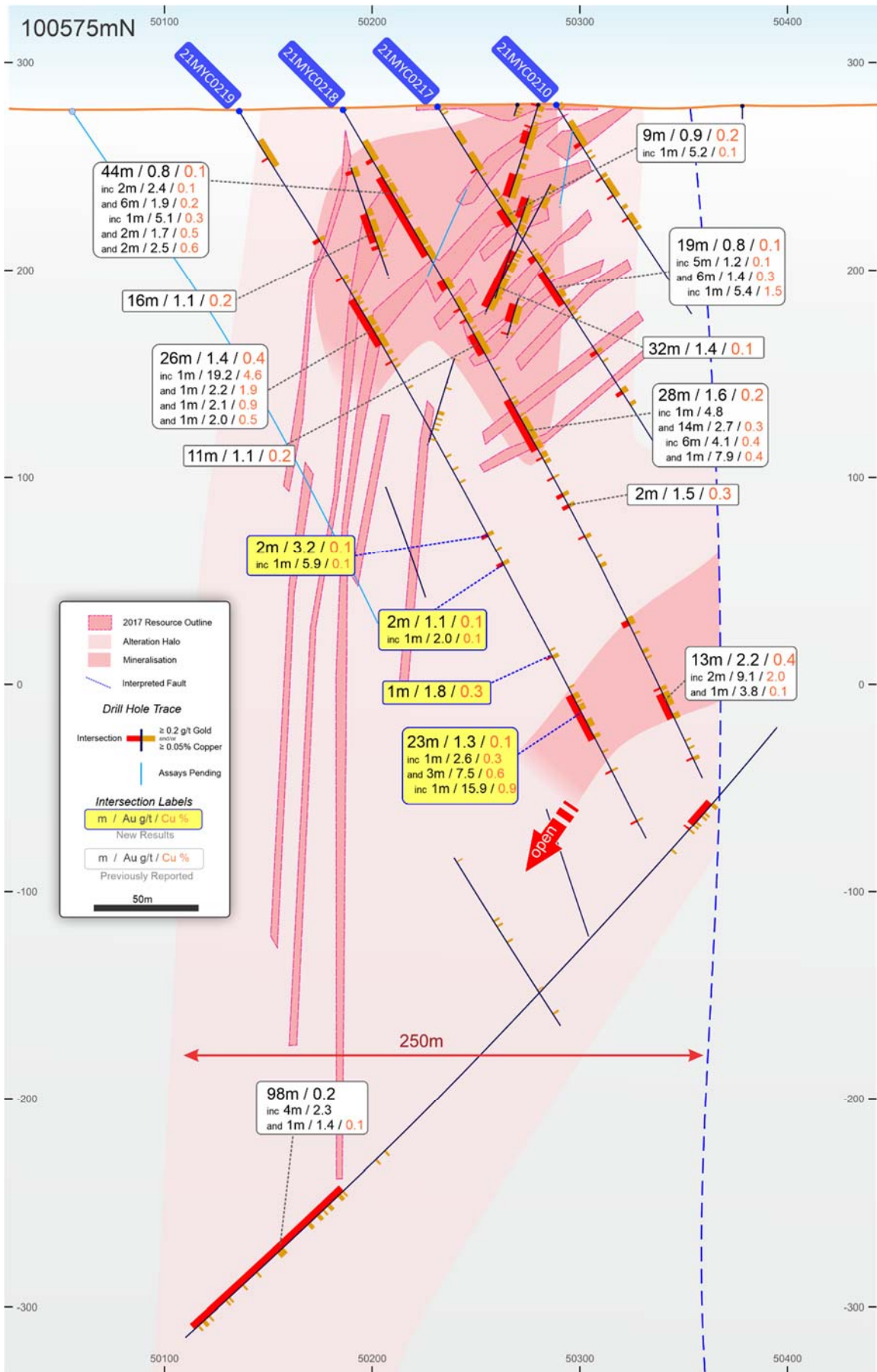
Figure 8: Minyari gold-copper-silver-cobalt deposit 100,575mN cross-section showing gold-copper drill intercepts, with the deposit open down dip and along strike/plunge.
