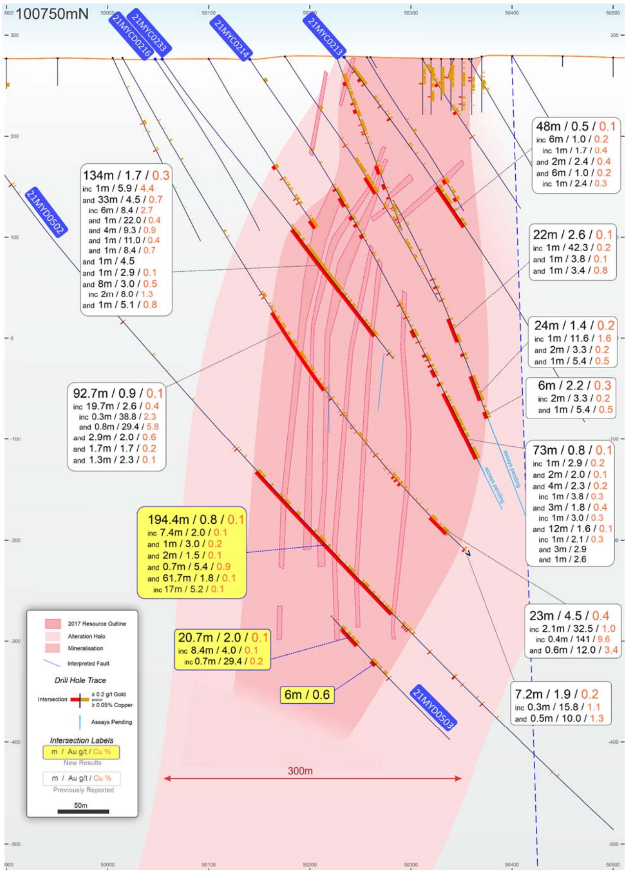
Figure 5: Minyari gold-copper-silver-cobalt deposit 100,750mN cross-section showing gold-copper drill intercepts, with the deposit open down dip and along strike/plunge.
