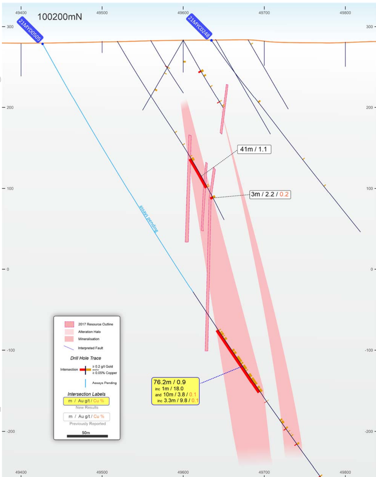
Figure 12: WACA gold-copper-silver-cobalt deposit 100,200mN cross-section showing gold-copper drill intercepts, with the deposit open down dip and along strike/plunge.
