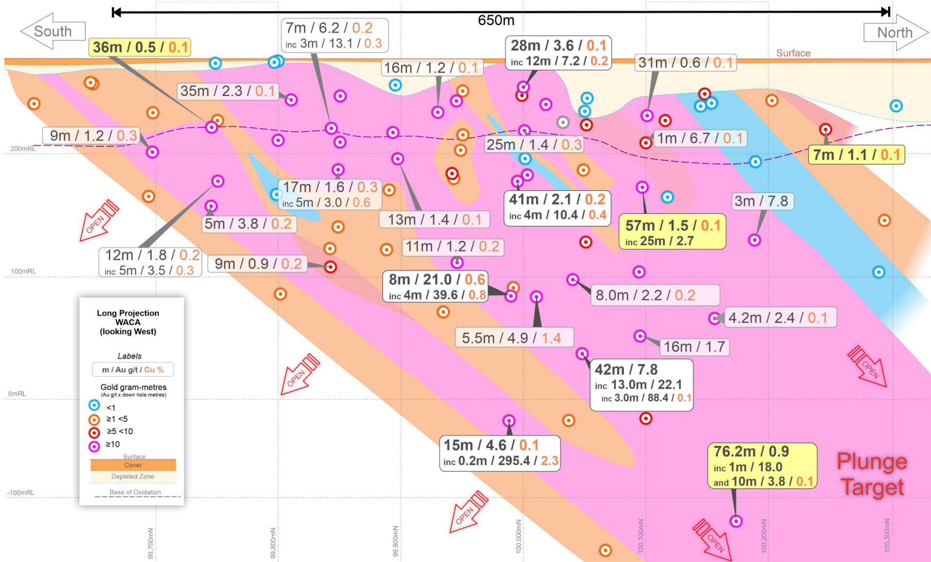
Figure 11: WACA Deposit Long Section showing drill holes pierce points and gold gram-metres (i.e. Au g/t x down hole metres) along a +650m strike length showing high-grade gold mineralisation open down dip / plunge to the northwest and potentially along strike.
