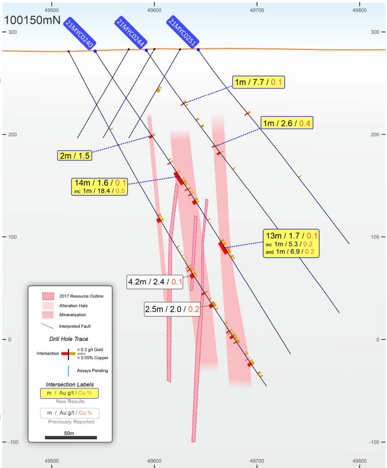
Figure 13: WACA gold-copper-silver-cobalt deposit 100,150mN cross-section showing gold-copper drill intercepts, with the deposit open down dip and along strike/plunge.
