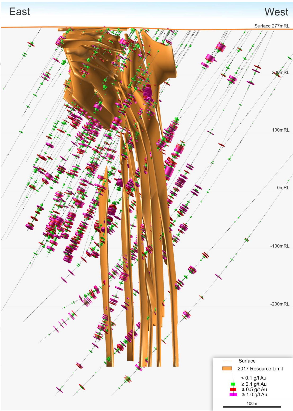
Figure 1: Minyari deposit cross-section view showing only the 2020 (3 holes) and 2021 drill hole gold intercepts which post-date the 2017 Mineral Resource (brown wireframes). Note the abundant mineralisation discovered to the east, west and between the 2017 resource, with the deposit still remaining open in several directions. NB: 100m Elevation grid (MGA mRL), looking toward Local 192° (or 160° MGA Zone 51).
