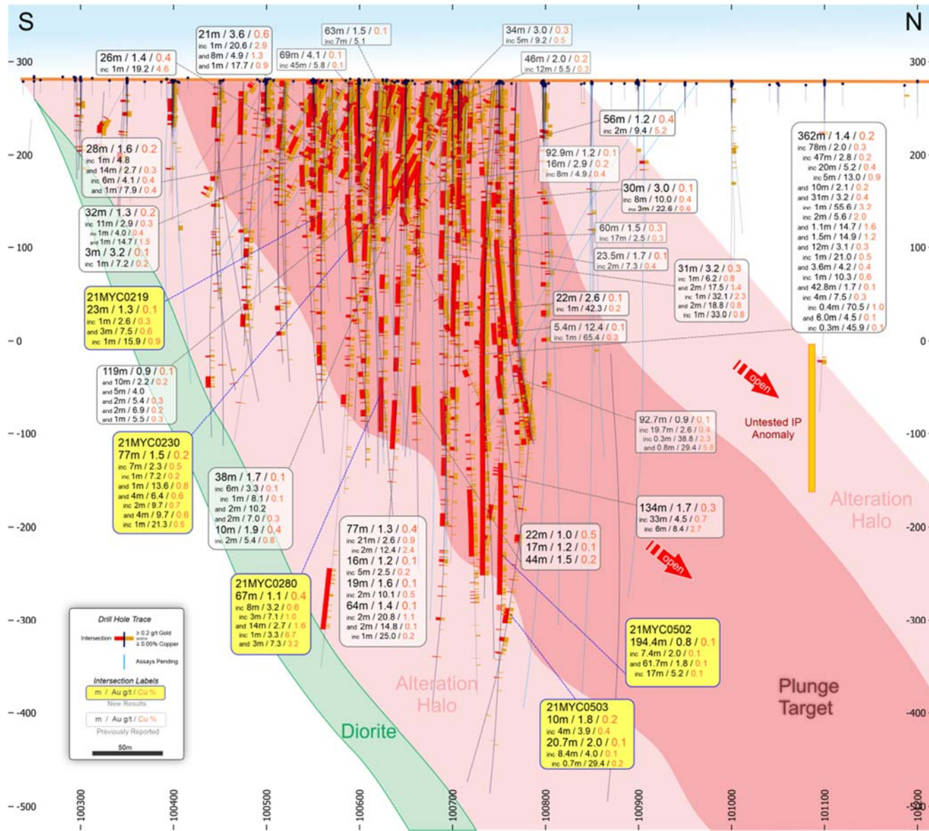
Figure 3: Minyari deposit Long Section view showing distribution of gold-copper mineralisation, and northern plunge target.
