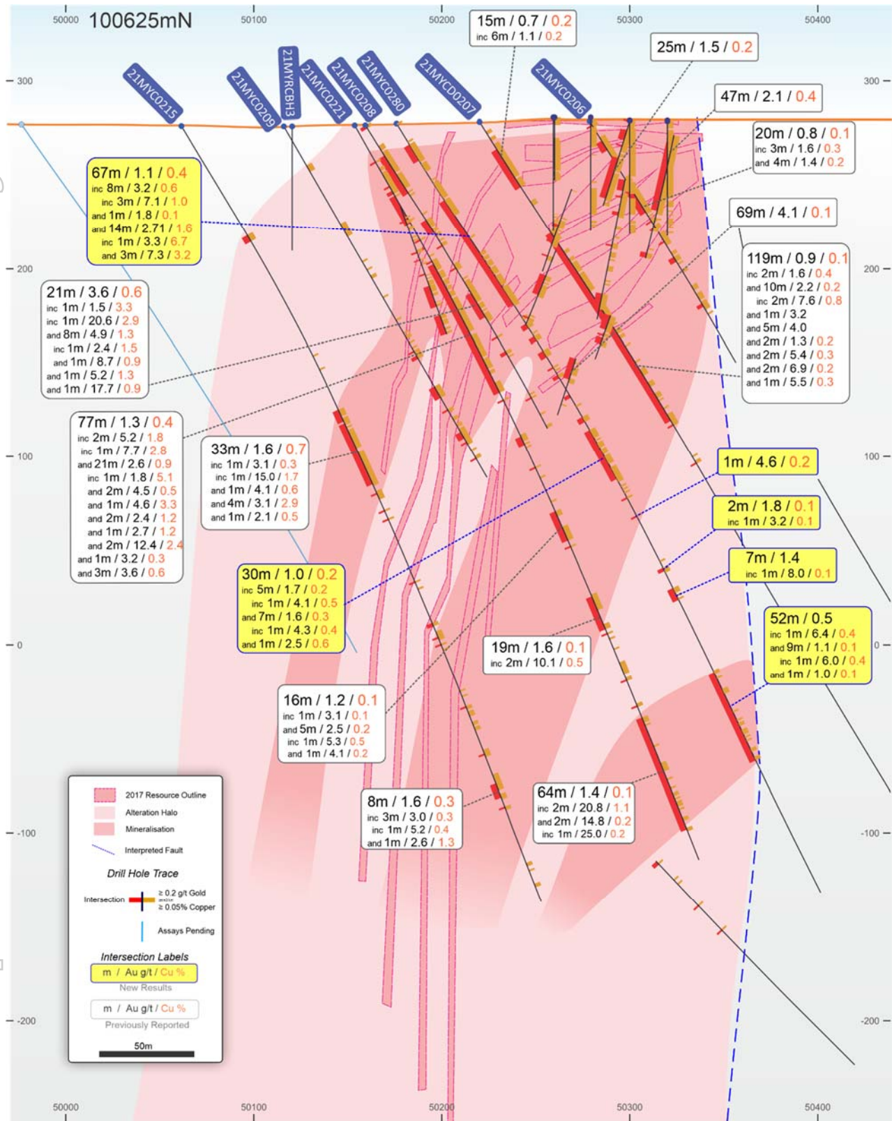
Figure 7: Minyari gold-copper-silver-cobalt deposit 100,625mN cross-section showing gold-copper drill intercepts, with the deposit open down dip and along strike/plunge.
