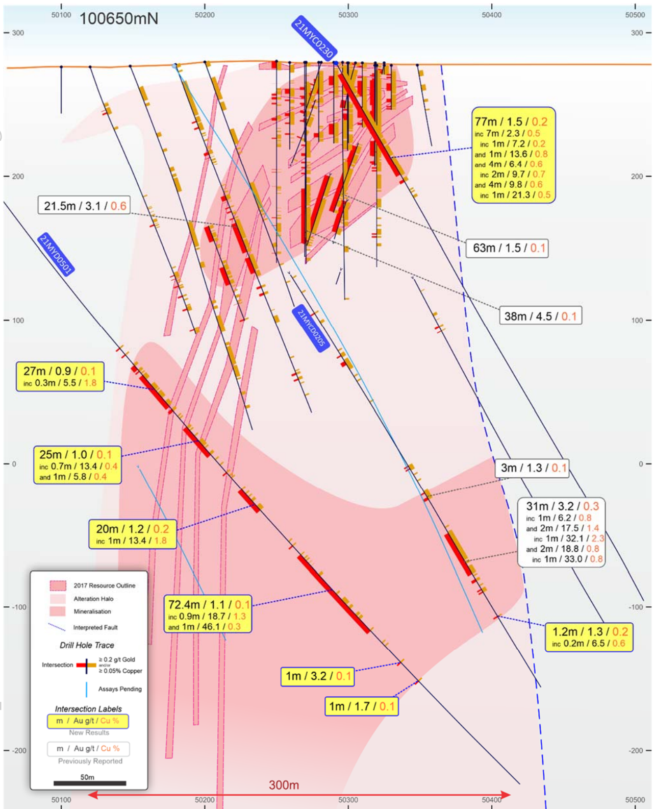
Figure 6: Minyari gold-copper-silver-cobalt deposit 100,650mN cross-section showing gold-copper drill intercepts, with the deposit open down dip and along strike/plunge.
