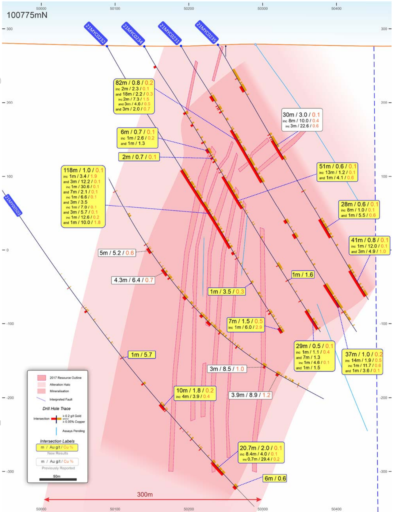
Figure 4: Minyari gold-copper-silver-cobalt deposit 100,775mN cross-section showing gold-copper drill intercepts, with the deposit open down dip and along strike/plunge.
