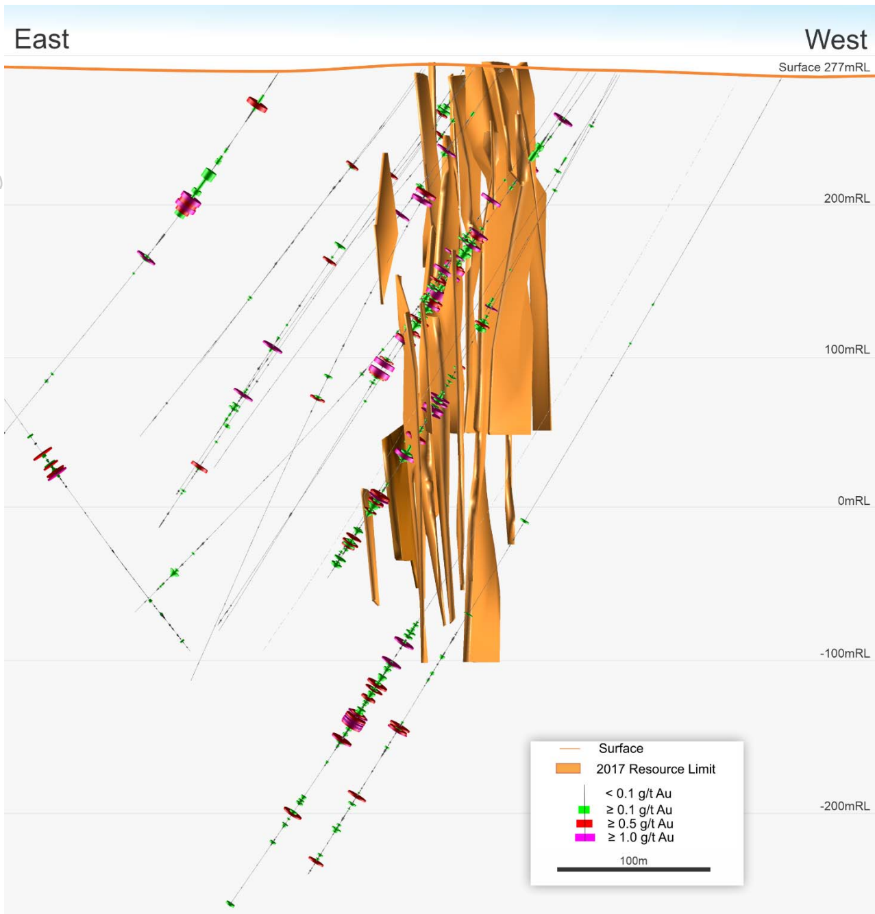
Figure 10: WACA deposit cross-section view showing only the 2020 (2 holes) and available 2021 drill hole gold intercepts which post-date the 2017 Mineral Resource (brown wireframes). Note the mineralisation discovered to the east, between and below the 2017 resource, with the deposit still remaining open in several directions. NB: 100m Elevation grid (MGA mRL), looking toward Local Grid 192° (or 160° MGA Zone 51).
