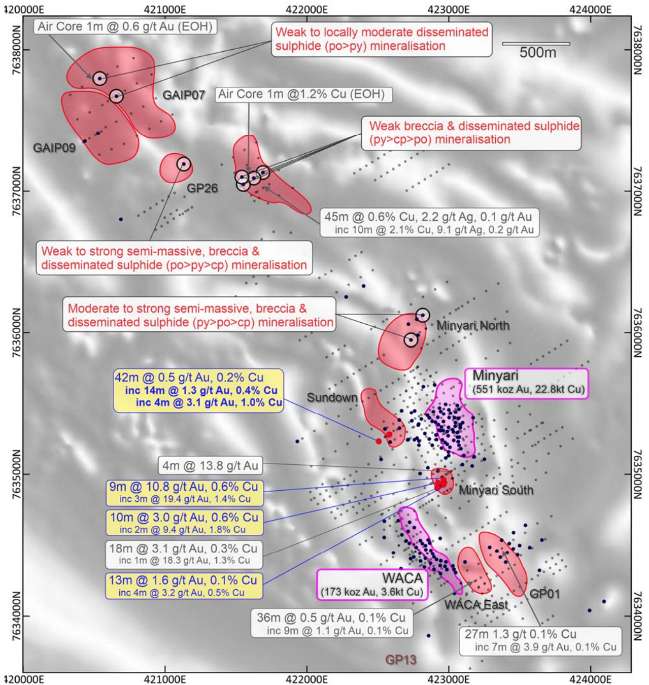
Figure 15: Map of the southern region of the Minyari Dome Project showing Minyari and WACA resource locations, Judes prospect and GAIP07-09 target locations, and drill hole maximum downhole gold and copper. NB: Over Airborne magnetic image (50m flight-line spacing at an altitude of 30m; grey-scale TMI-RP) and Regional GDA2020 / MGA Zone 51 co-ordinates, 1km grid.
