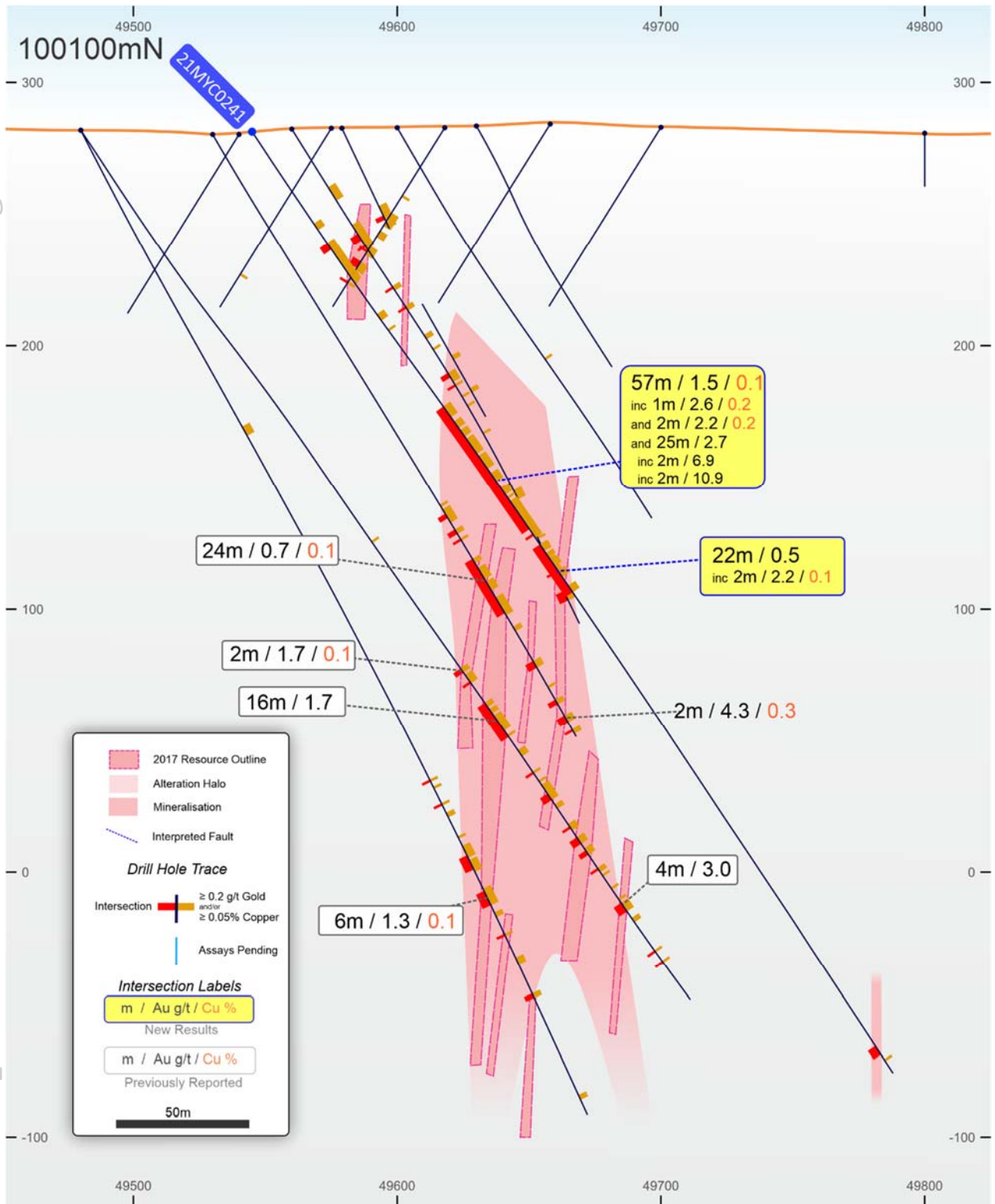
Figure 14: WACA gold-copper-silver-cobalt deposit 100,100mN cross-section showing gold-copper drill intercepts, with the deposit open down dip and along strike/plunge.
