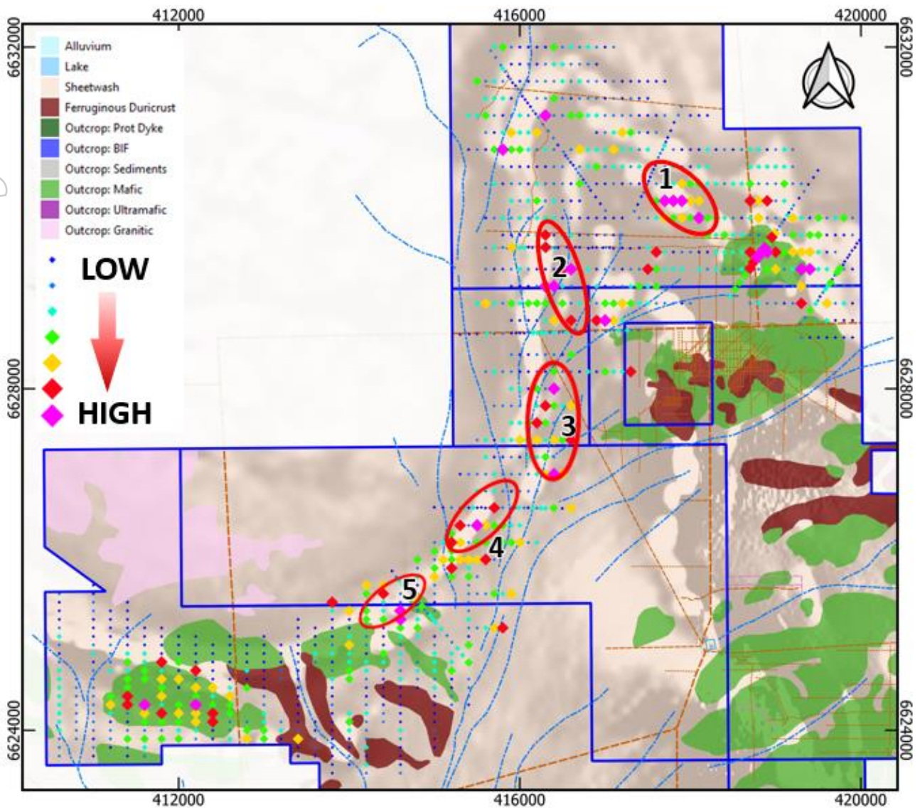
Figure 8: Log Additive Indices Ni+Cu (LAI_Ni Cu) on domained UFF soils
