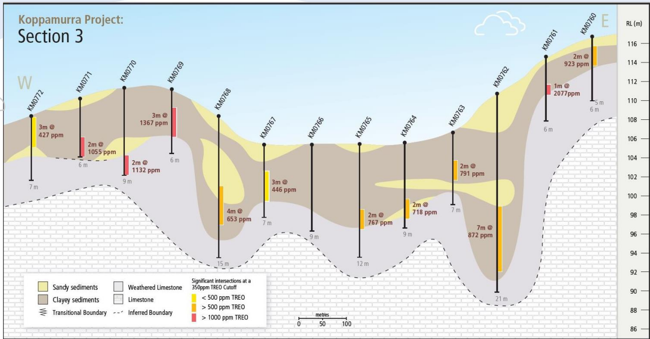
Figure 4 – Cross Section 3
