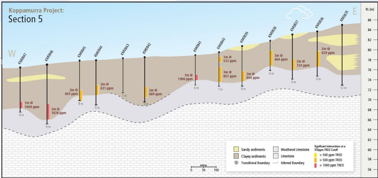
Figure 6 – Cross Section 5
