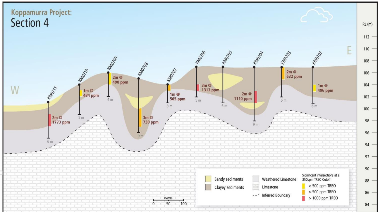
Figure 5 – Cross Section 4
