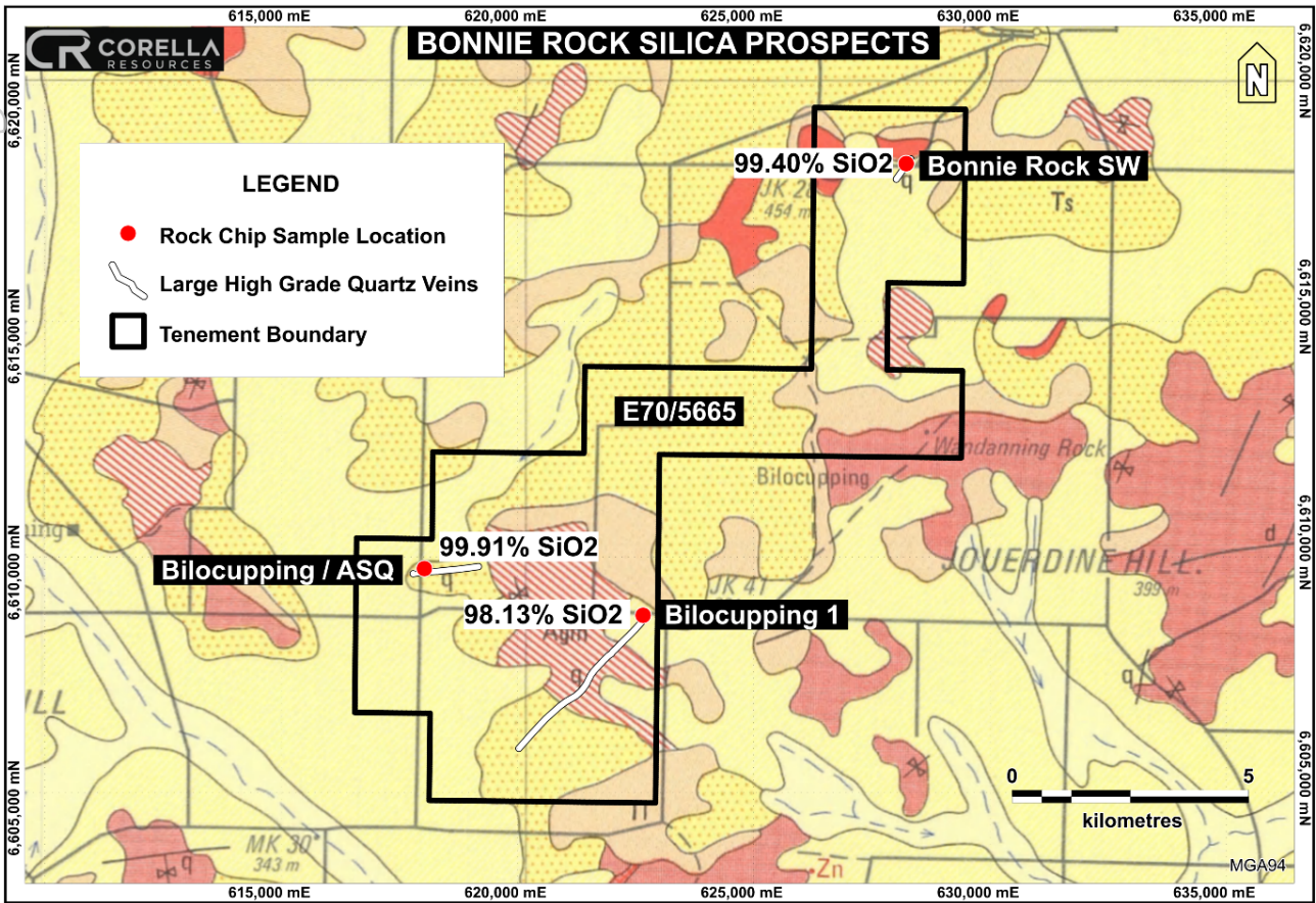
Figure 6: Location map showing the high-grade silica (quartz vein) prospects at the Bonnie Rock Silica Project
