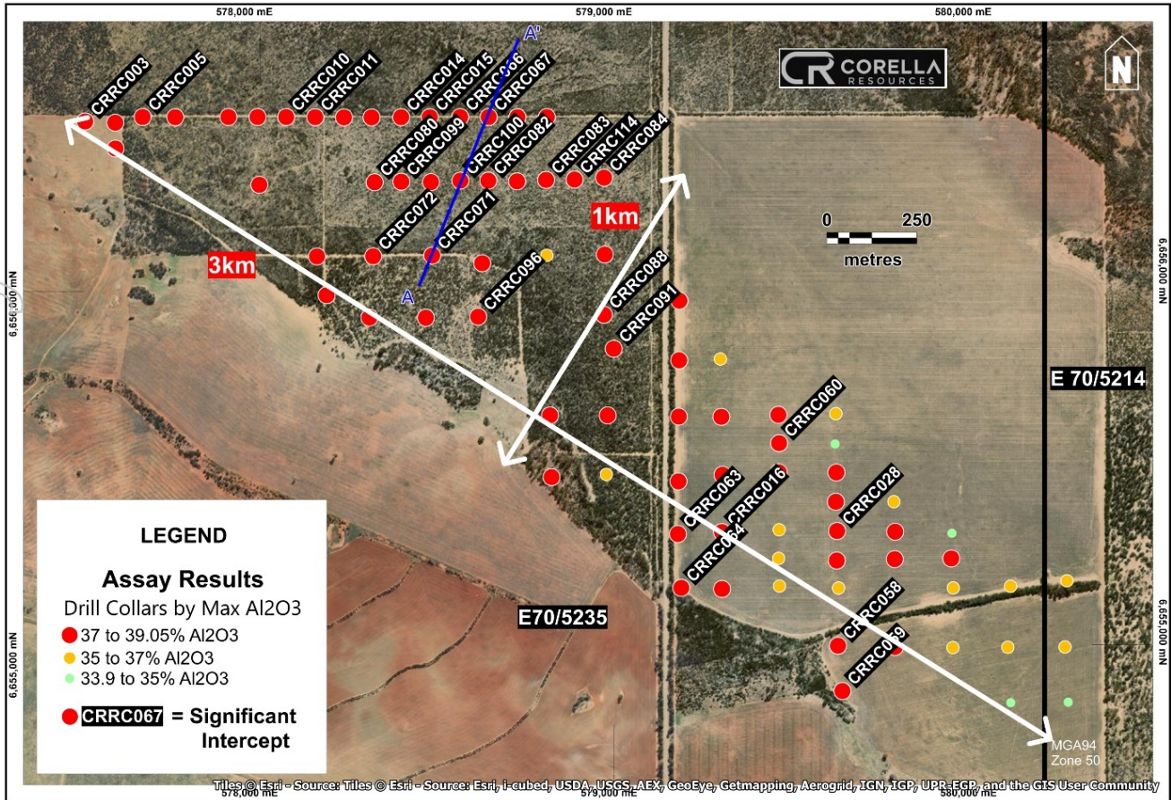
Figure 4: Map of the Tampu drillholes coloured by Al 2 O 3 content
