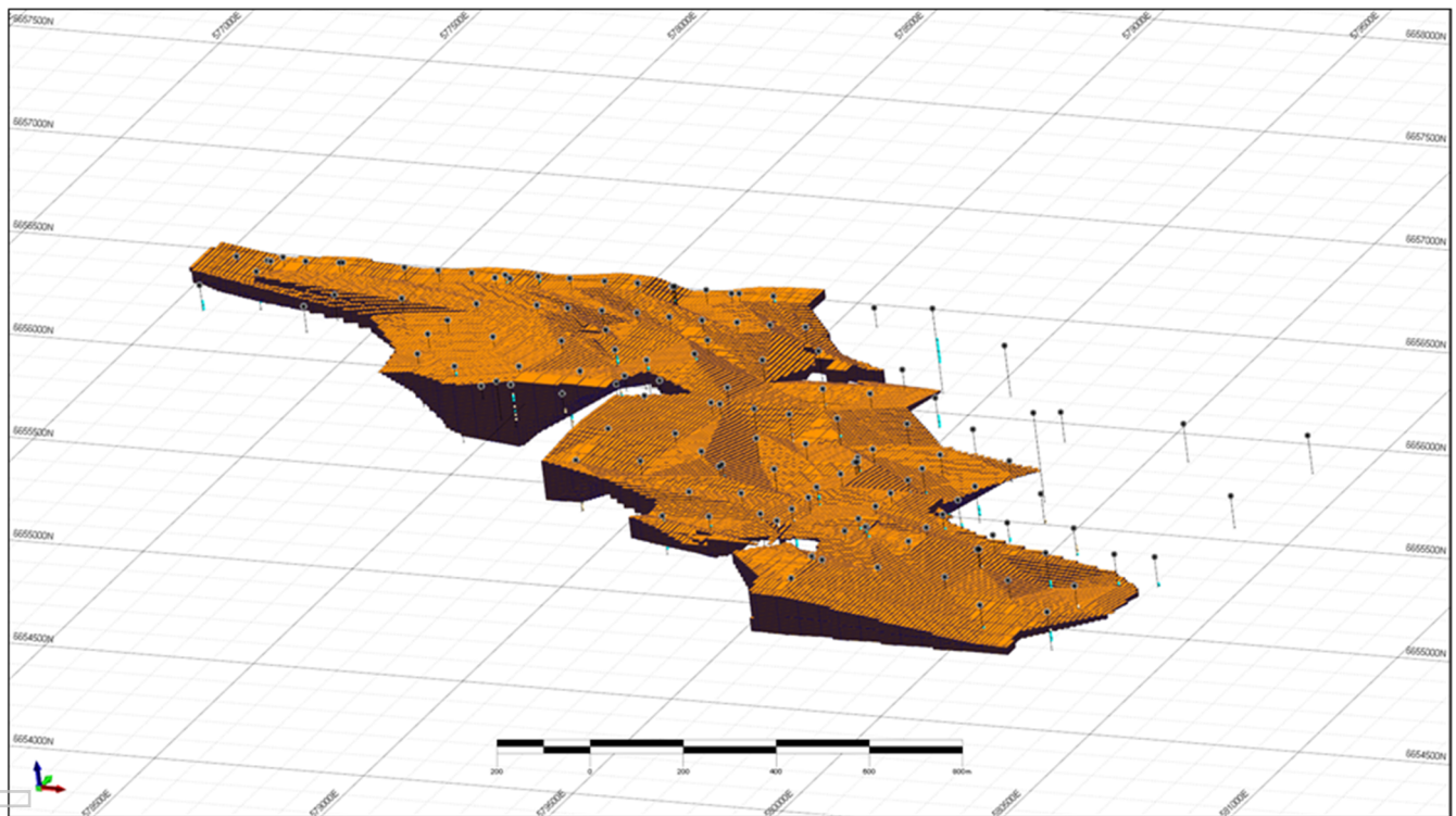
Figure 1 – Tampu Resource Block Model Oblique View (looking north & using a 1.2\% Fe 2 O 3 cut-off)
