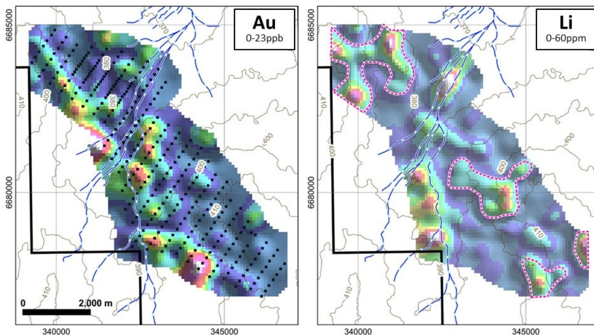
Figure 9 – Gold (left) and Lithium anomalism throughout the Pianto survey area. Other Li pathfinder elements show similar anomaly distributions, suggesting a basement source. Projection GDA94 MGA Zone 51.
