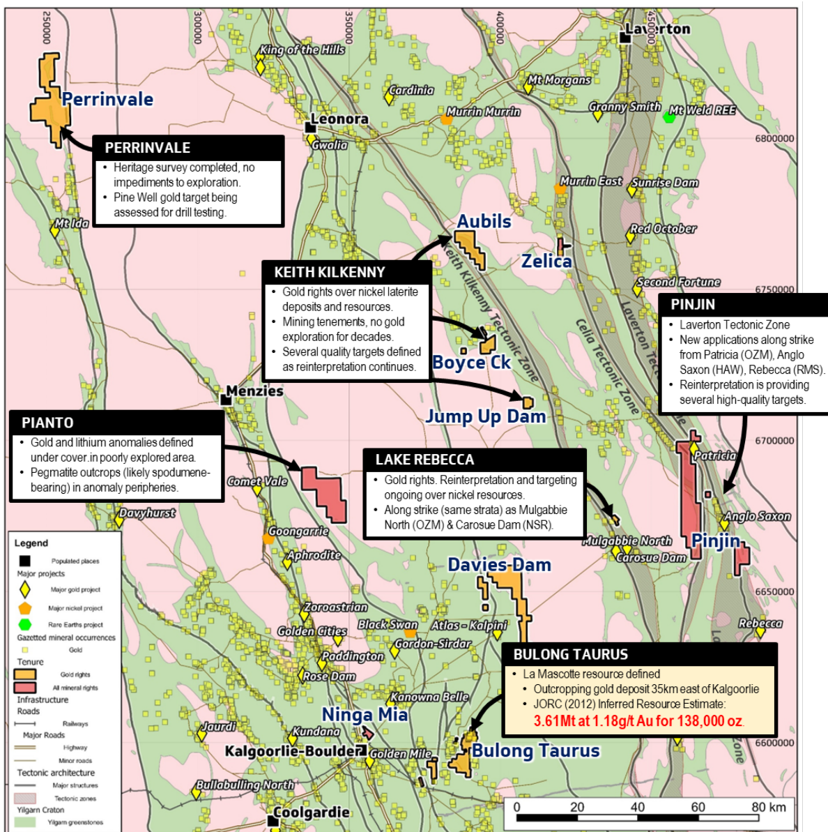
Figure 1 – KalGold's projects in the Eastern Goldfields of WA, showing current work activities overlaid on regional geology, showing granite/greenstone distributions and major faults and tectonic zones. Towns, railways, and major roads also shown. Note that aspects of this diagram reflect events subsequent to the reporting period as addressed in this report.
