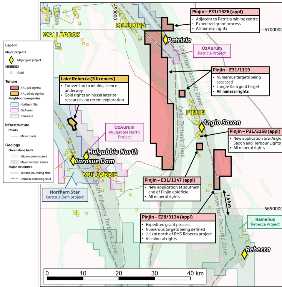
Figure 5 – KalGold’s Pinjin Project (in the Laverton Tectonic Zone) and Lake Rebecca Project (in the Keith Kilkenny Tectonic Zone), south-eastern Eastern Goldfields. The region is currently the focus of many companies. Projection GDA94 MGA Zone 51.
