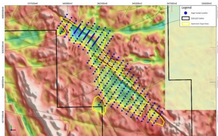
Figure 6 – Pianto auger program sample locations over conceptual exploration target areas (E29/1125). Projection GDA94 MGA Zone 51.
