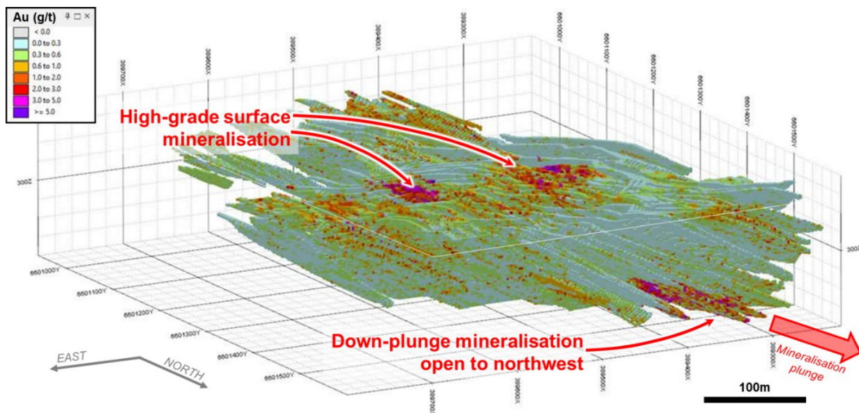
Figure 7 – Oblique view of the La Mascotte block model, looking downwards towards the southwest. Note high grade mineralisation near surface and open at depth down-plunge. Projection GDA94 MGA Zone 51.
