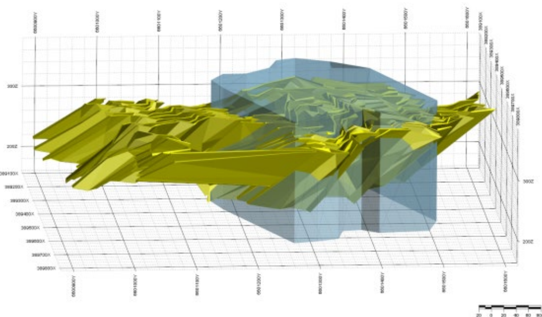
Figure 4 – Oblique view, looking to the west, of the 3D model of gold mineralisation that is in progress at La Mascotte (yellow wireframes). Work is in progress. The blue vertical wireframe is an encompassing block that represents the extent of modelling for the pre-JORC resource in the 1990s. Mineralisation modelled beyond this extent is supported by additional drilling undertaken by KalGold since listing in November 2021.
