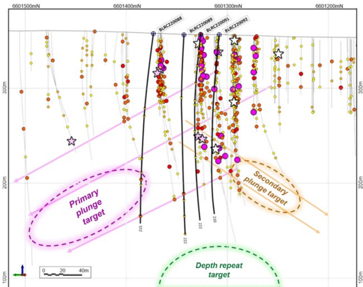
Figure 8 – Long section of extensive gold mineralisation at La Mascotte (looking eastward towards 070°), showing gold intercepts that define a north-westerly plunge. Refined targets are shown (see text for details). Note that the section plane is very thick, and the Primary Plunge Target (pink) is to the west or towards the viewer in this diagram. The Secondary Plunge Target is located immediately south of the deeper high-grade zone, and the Depth Repeat Target is located directly underneath the main deep high-grade zones.
