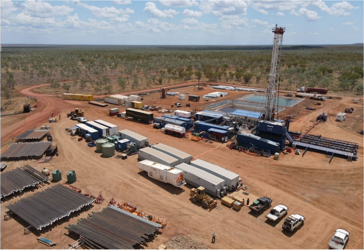
Carpentaria-3H Drilling Operations
